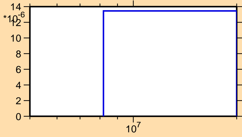
\sigma vs. E for ^{108}\text{Sb}(n,\text{pt})
