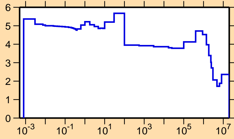
\sigma vs. E for ^{108}\text{Sb}(n,\text{el.})
