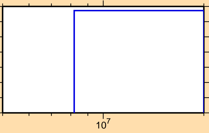
\sigma vs. E for ^{108}\text{Sb}(n,\text{pt})
