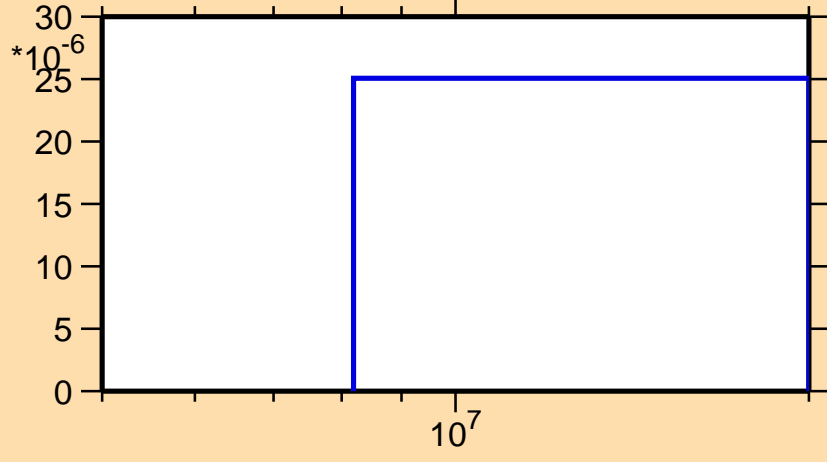
\sigma vs. E for ^{108}\text{Sb}(n,\text{nd})
