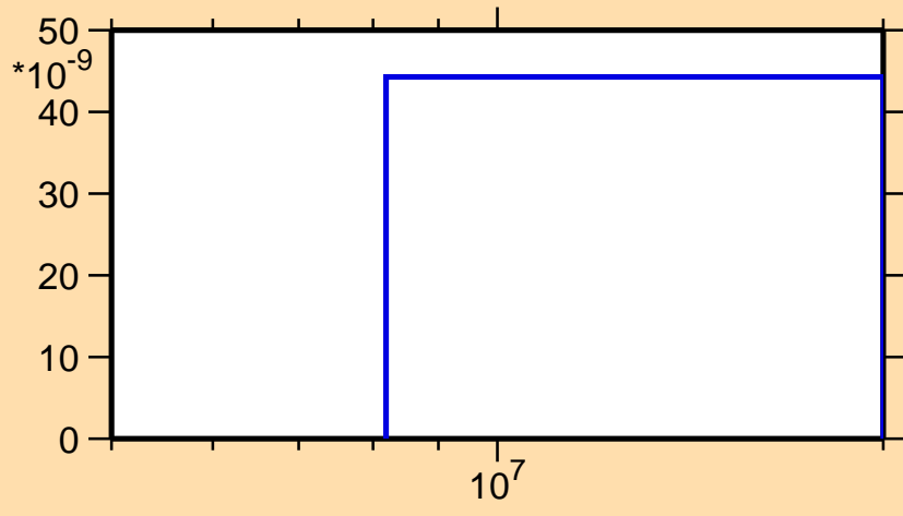
\sigma vs. E for ^{108}\text{Sb}(n,2n\alpha)
