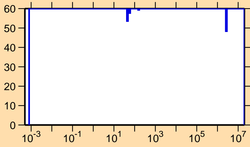
\Delta\sigma/\sigma vs. E for ^{109}\text{Sb}(n,\gamma)
