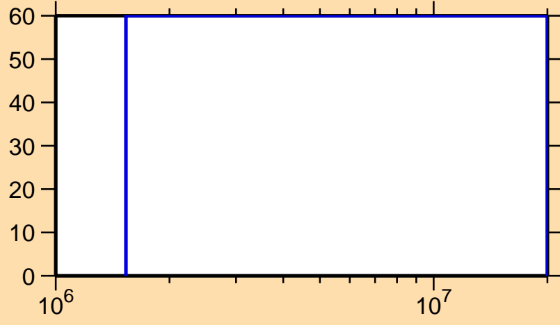
\Delta\sigma/\sigma vs. E for ^{109}\text{Sb}(n,n\text{cont.})
