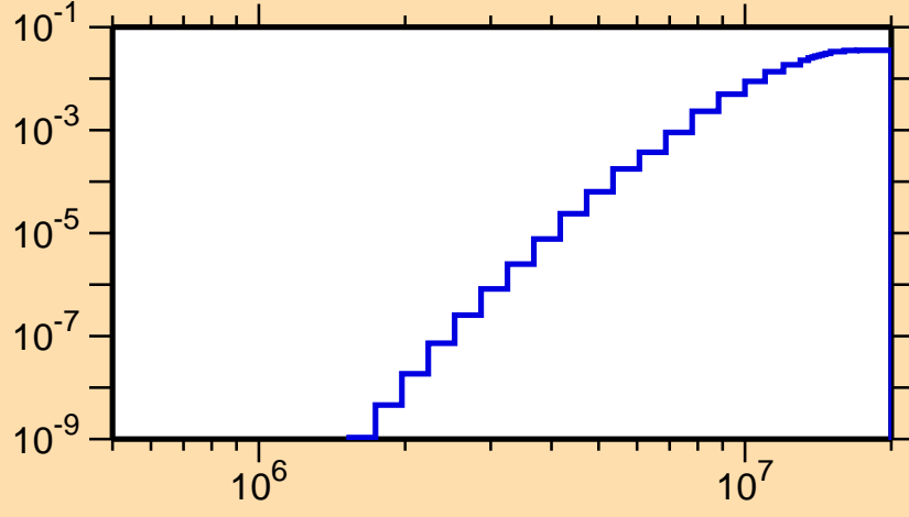
\sigma vs. E for ^{109}\text{Sb}(n,d)
