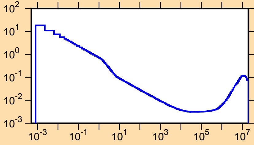
\sigma vs. E for ^{109}\text{Sb}(n,\alpha)
