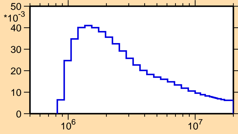
\sigma vs. E for ^{109}\text{Sb}(n,n_3)
