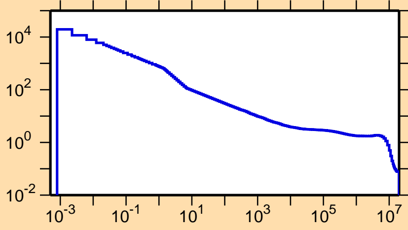
\sigma vs. E for ^{109}\text{Sb}(n,p)
