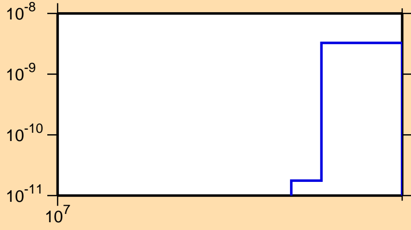
\sigma vs. E for ^{109}\text{Sb} (mt 34)
