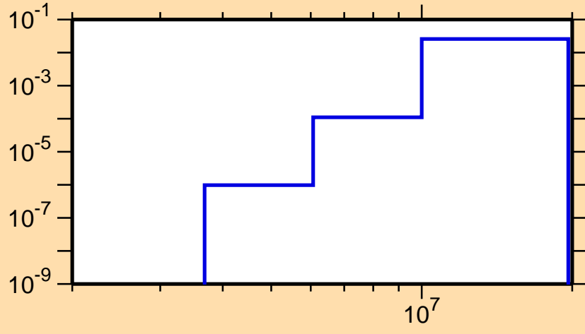
\sigma vs. E for ^{109}\text{Sb}(n,n\alpha)
