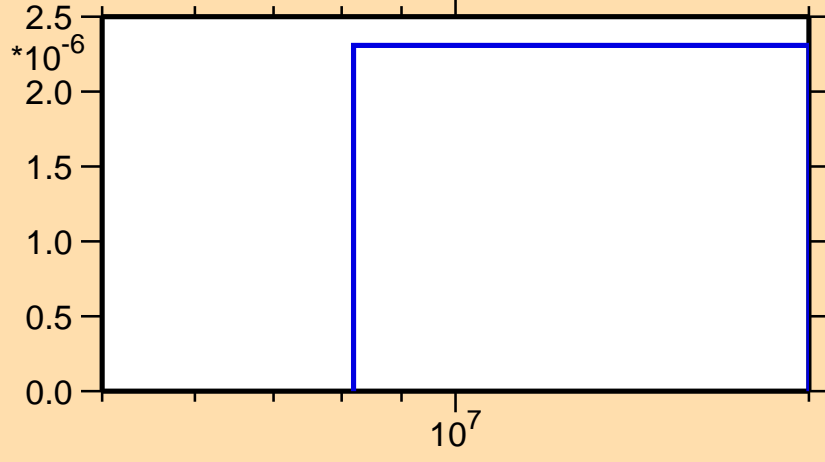
\sigma vs. E for ^{109}\text{Sb}(n,nd)
