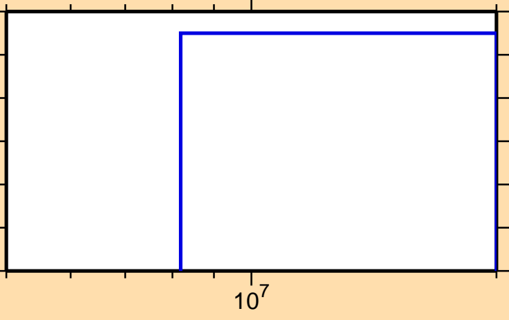
\sigma vs. E for ^{109}\text{Sb}(n,2np)
