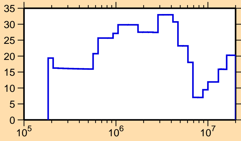
\Delta\sigma/\sigma vs. E for ^{110}\text{Sb}(n,\text{el.})
