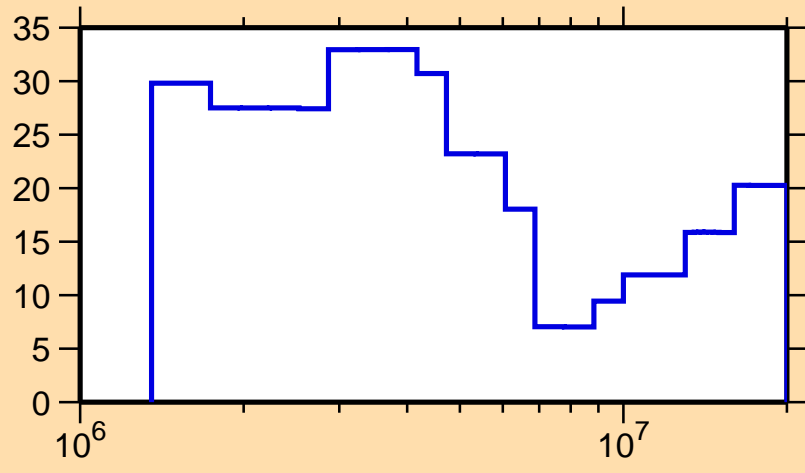
\Delta\sigma/\sigma vs. E for ^{110}\text{Sb}(n,el.)
