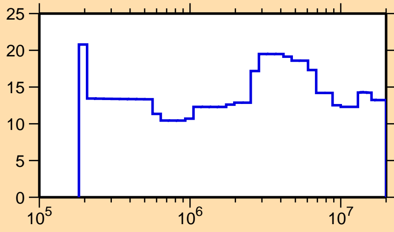
\Delta\sigma/\sigma vs. E for ^{110}\text{Sb}(n,\text{nonel.})
