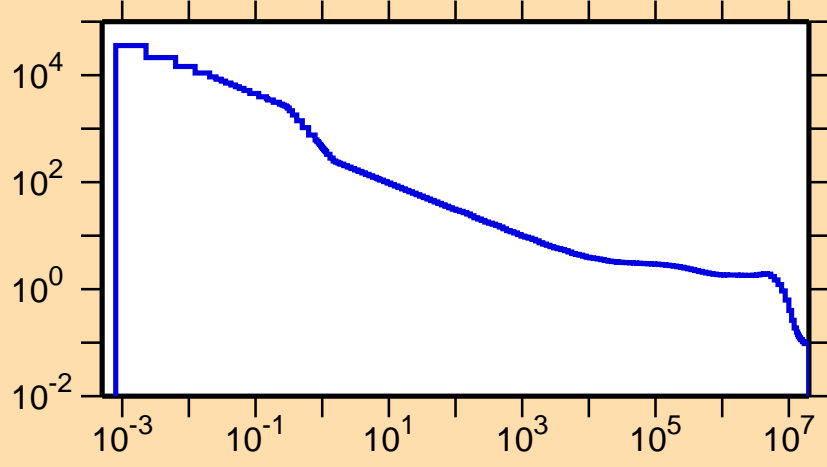
\sigma vs. E for ^{110}\text{Sb}(n,p)
