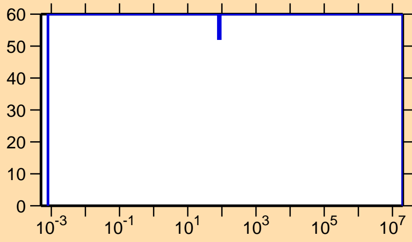
\Delta\sigma/\sigma vs. E for ^{110}\text{Sb}(n,\gamma)
