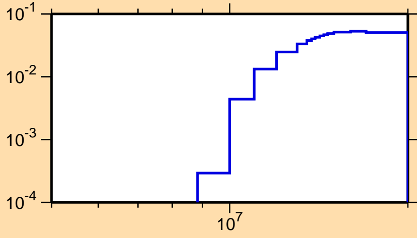
\sigma vs. E for ^{110}\text{Sb}(n,2n)
