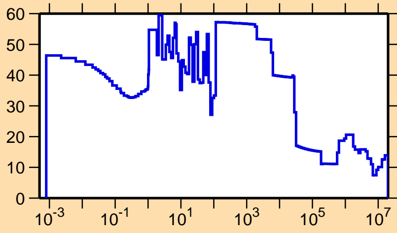
\Delta\sigma/\sigma vs. E for ^{110}\text{Sb}(n,\text{tot.})
