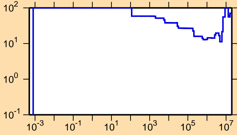
\Delta\sigma/\sigma vs. E for ^{110}\text{Sb}(n,p)
