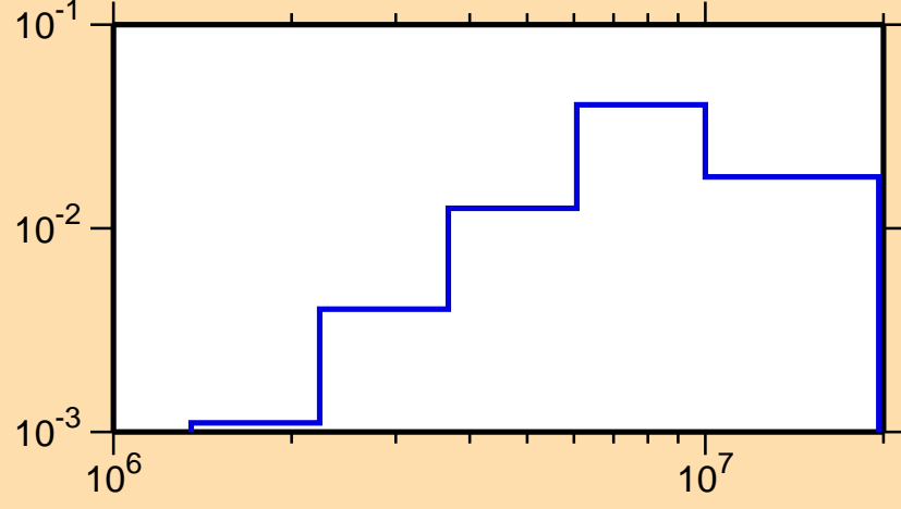
\sigma vs. E for ^{110}\text{Sb}(n,n\text{cont.})
