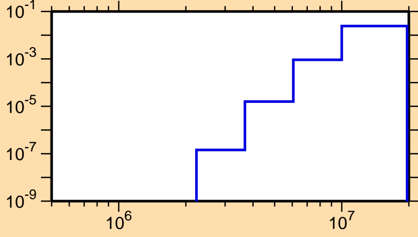
\sigma vs. E for ^{110}\text{Sb}(n,d)
