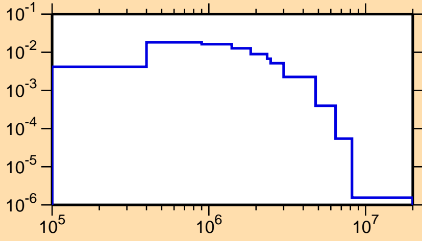
\sigma vs. E for ^{110}\text{Sb}(n,n_1)
