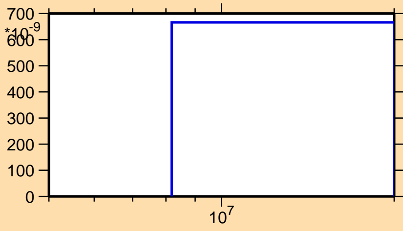
\sigma vs. E for ^{110}\text{Sb}(n,pt)
