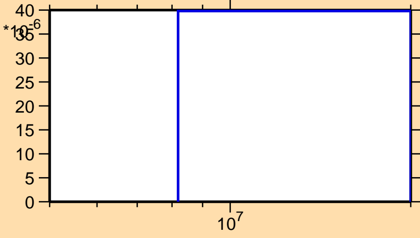
\sigma vs. E for ^{110}\text{Sb}(n,pd)
