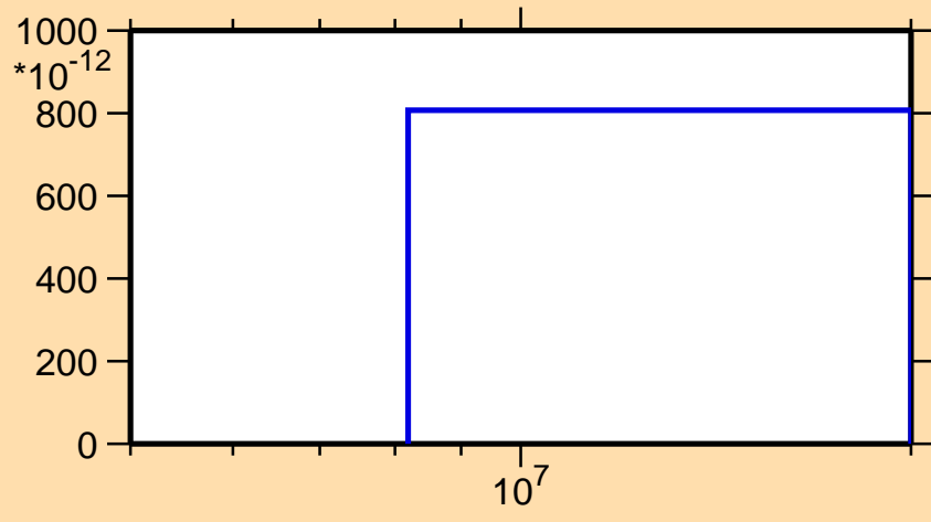
\sigma vs. E for ^{110}\text{Sb}(n,nt)
