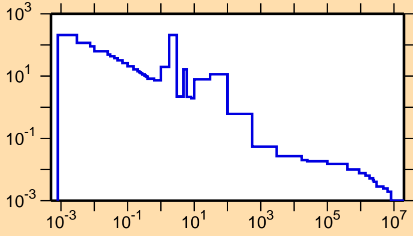
\sigma vs. E for ^{110}\text{Sb}(n,\gamma)
