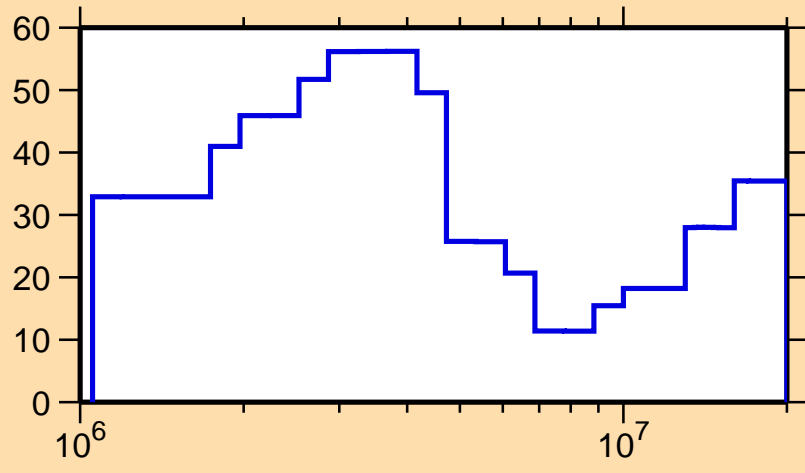
\Delta\sigma/\sigma vs. E for ^{112}\text{Sb}(n,el.)
