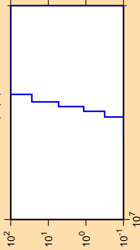
\Delta\sigma/\sigma vs. E for ^{112}\text{Sb}(n,pt)
