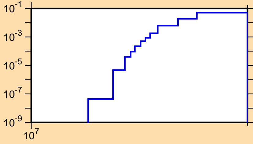
\sigma vs. E for ^{112}\text{Sb}(n,2np)
