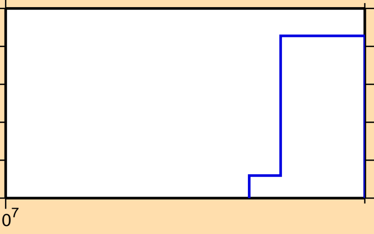
\sigma vs. E for ^{112}\text{Sb}(n,nt)
