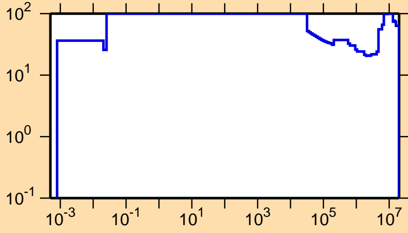
\Delta\sigma/\sigma vs. E for ^{112}\text{Sb}(n,p)
