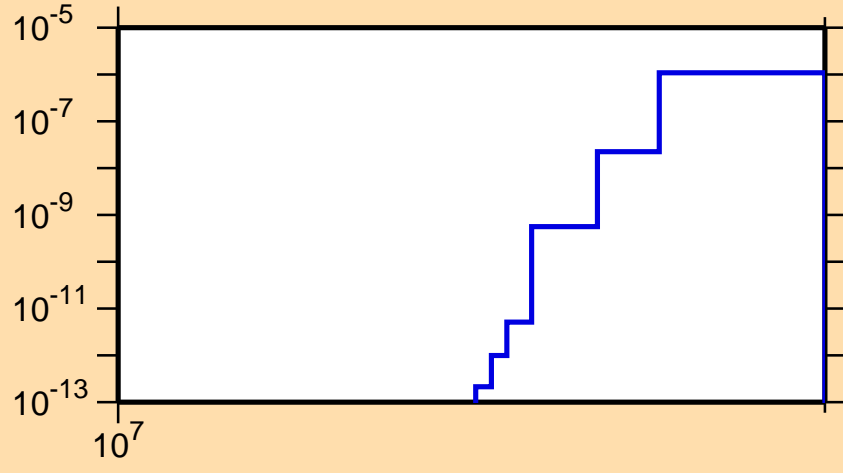
\sigma vs. E for ^{112}\text{Sb}(n,pt)
