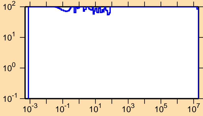
\Delta\sigma/\sigma vs. E for ^{112}\text{Sb}(n,\gamma)
