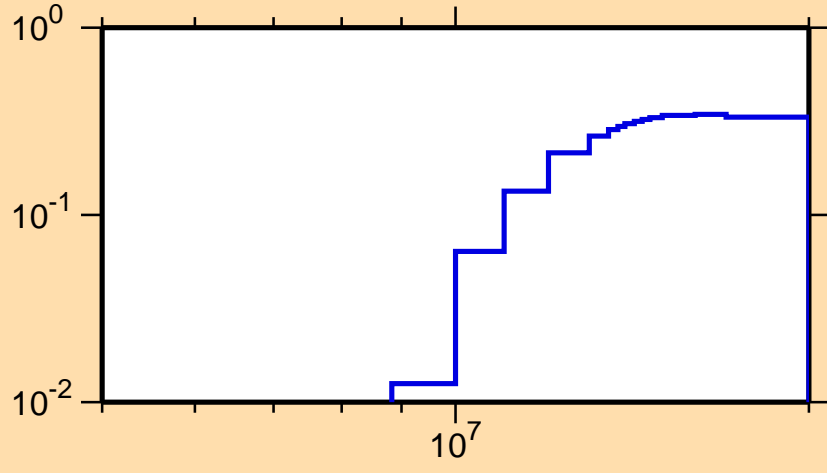
\sigma vs. E for ^{112}\text{Sb}(n,2n)
