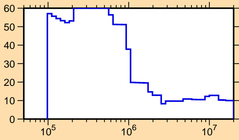
\Delta\sigma/\sigma vs. E for ^{112}\text{Sb}(n,\text{nonel.})
