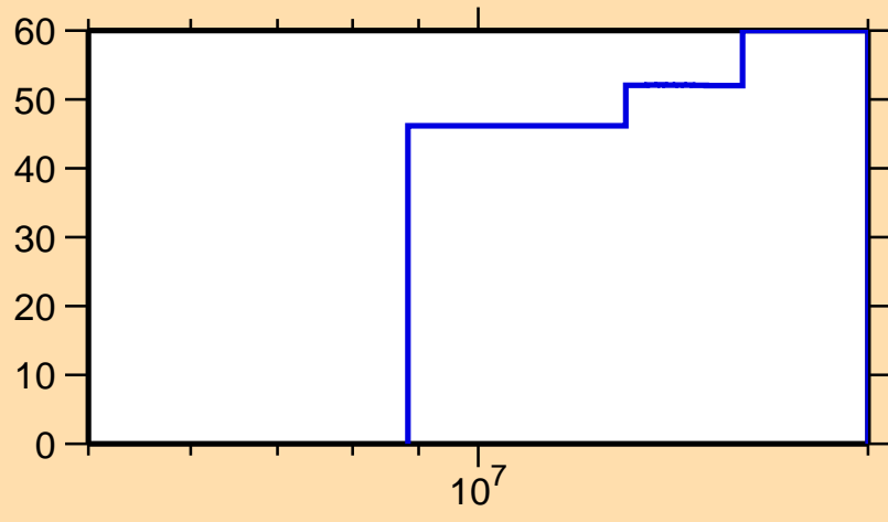
\Delta\sigma/\sigma vs. E for ^{112}\text{Sb}(n,2n)
