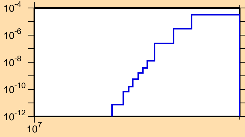
\sigma vs. E for ^{112}\text{Sb}(n,2n\alpha)
