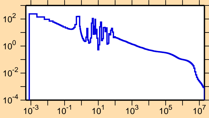
\sigma vs. E for ^{112}\text{Sb}(n,\gamma)
