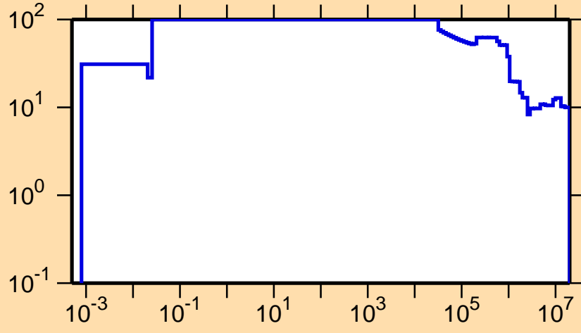
\Delta\sigma/\sigma vs. E for ^{112}\text{Sb}(n,\text{nonel.})
