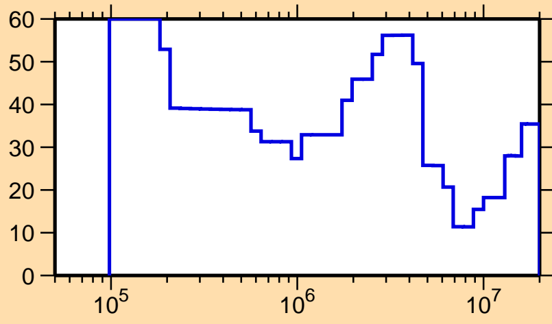
\Delta\sigma/\sigma vs. E for ^{112}\text{Sb}(n,\text{el.})
