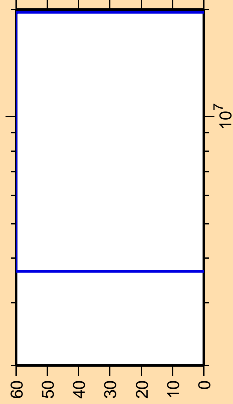
\Delta\sigma/\sigma vs. E for ^{112}\text{Sb}(n,n\alpha)
