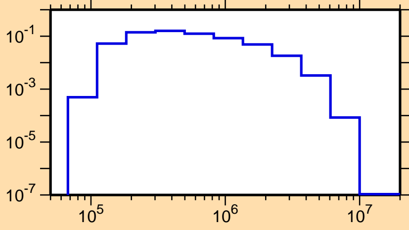
\sigma vs. E for ^{112}\text{Sb}(n,n_1)
