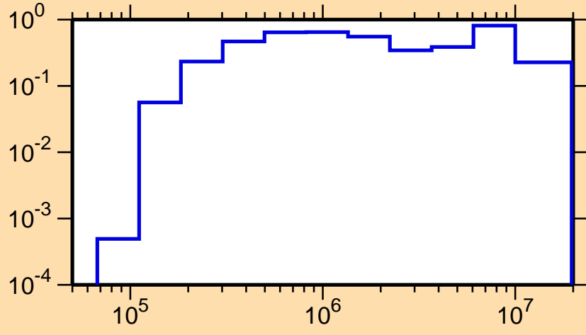
\sigma vs. E for ^{112}\text{Sb}(n,\text{inel.})
