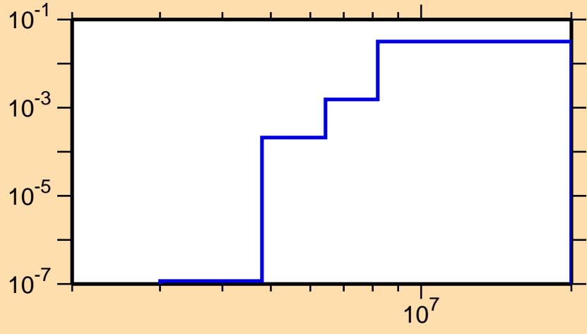
\sigma vs. E for ^{112}\text{Sb}(n,n\alpha)
