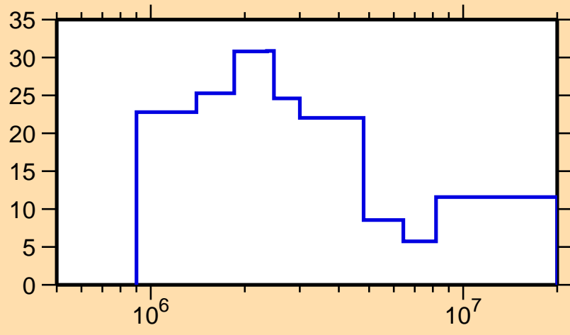
\Delta\sigma/\sigma vs. E for ^{112}\text{Sb}(n, tot.)
