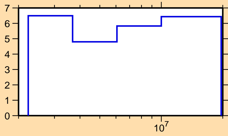
\Delta\sigma/\sigma vs. E for ^{113}\text{Sb}(n,\text{el.})
