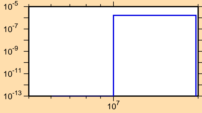
\sigma vs. E for ^{113}\text{Sb}(n,\text{He3})
