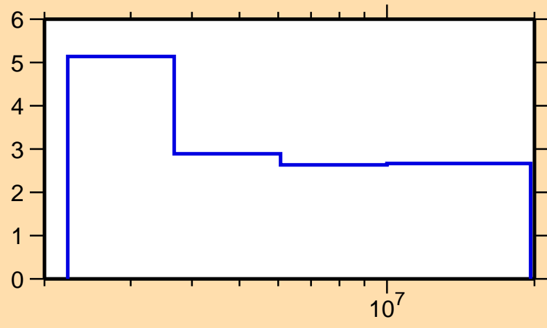
\Delta\sigma/\sigma vs. E for ^{113}\text{Sb}(n,\text{nonel.})
