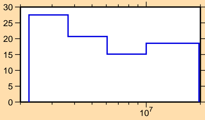
\Delta\sigma/\sigma vs. E for ^{113}\text{Sb}(n,n\text{cont.})
