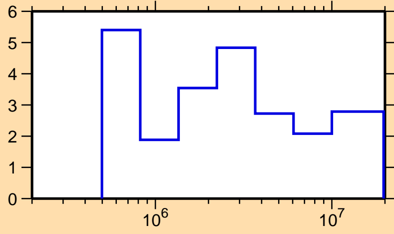
\Delta\sigma/\sigma vs. E for ^{113}\text{Sb}(n,\text{tot.})
