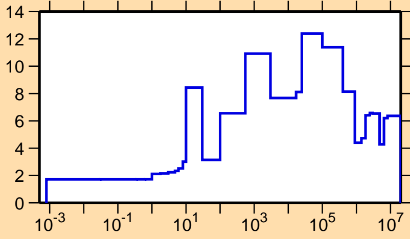
\Delta\sigma/\sigma vs. E for ^{113}\text{Sb}(n,el.)
