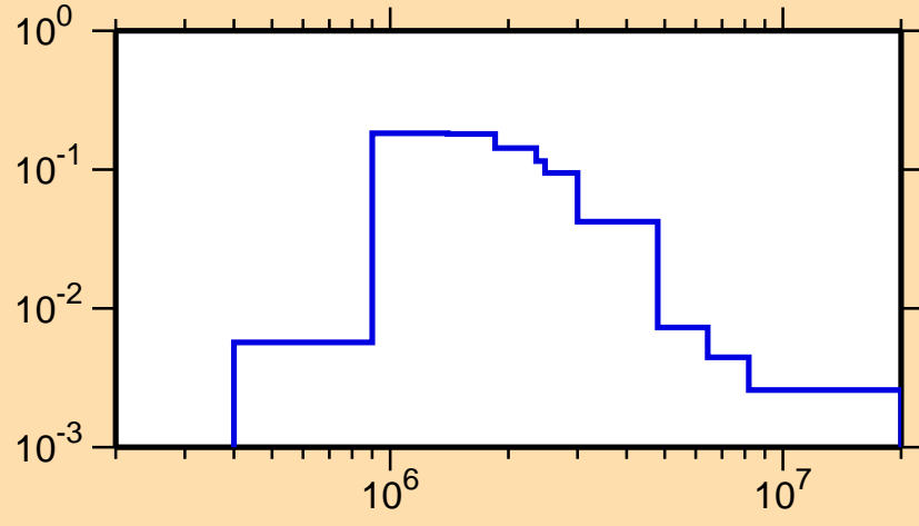
\sigma vs. E for ^{113}\text{Sb}(n,n_2)
