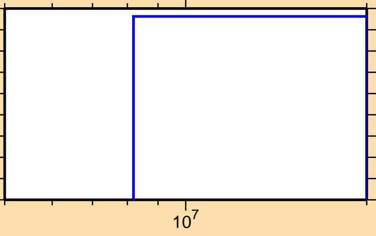
\sigma vs. E for ^{113}\text{Sb} (mt 45)
