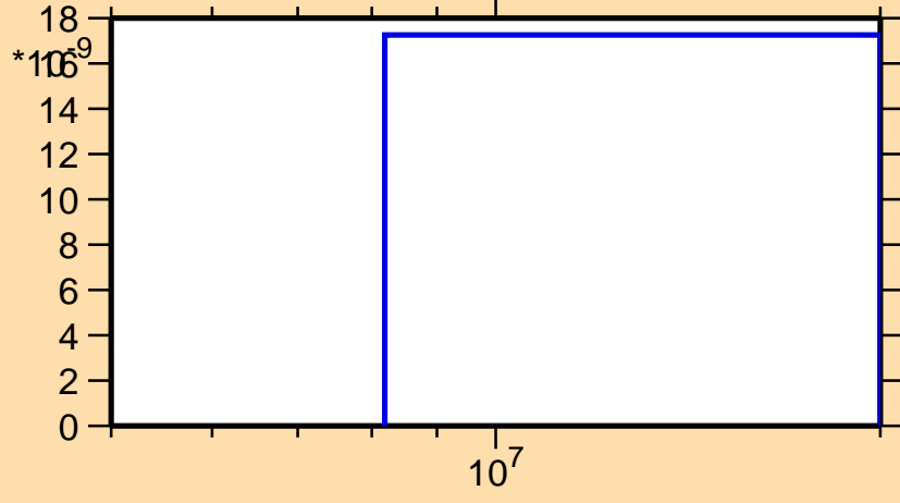
\sigma vs. E for ^{113}\text{Sb} (mt 45)
