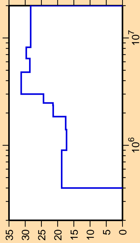
\Delta\sigma/\sigma vs. E for ^{113}\text{Sb}(n,n_2)
