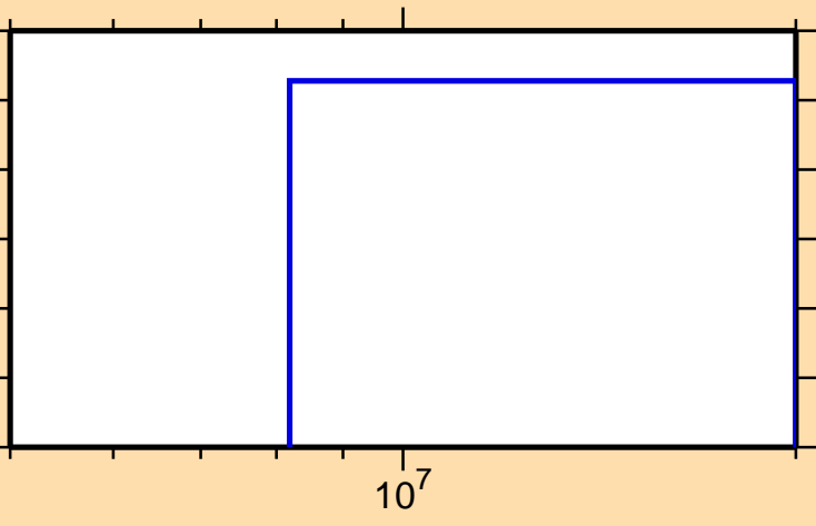
\sigma vs. E for ^{113}\text{Sb}(n,2np)
