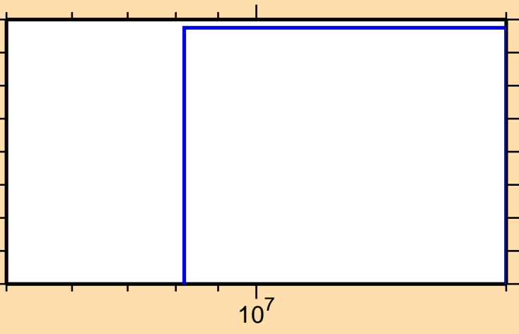
\sigma vs. E for ^{114}\text{Sb}(n,\text{nd})
