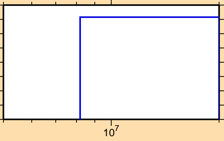
\sigma vs. E for ^{114}\text{Sb}(n,3n)
