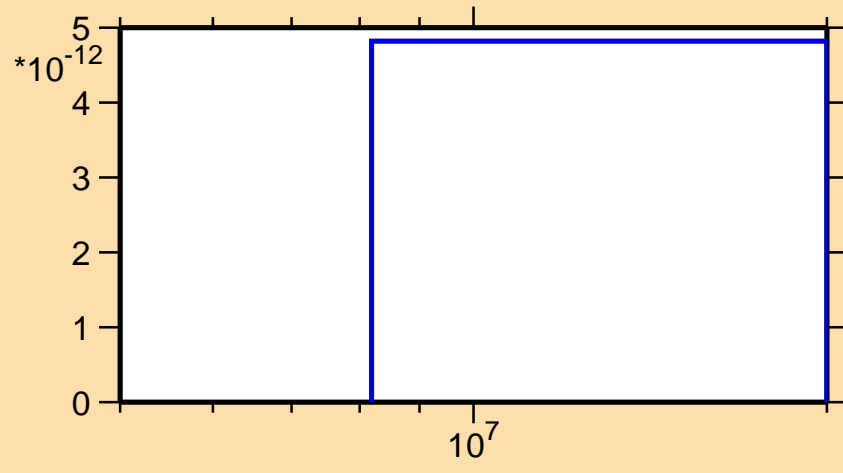
\sigma vs. E for ^{114}\text{Sb}(\text{mt } 34)
