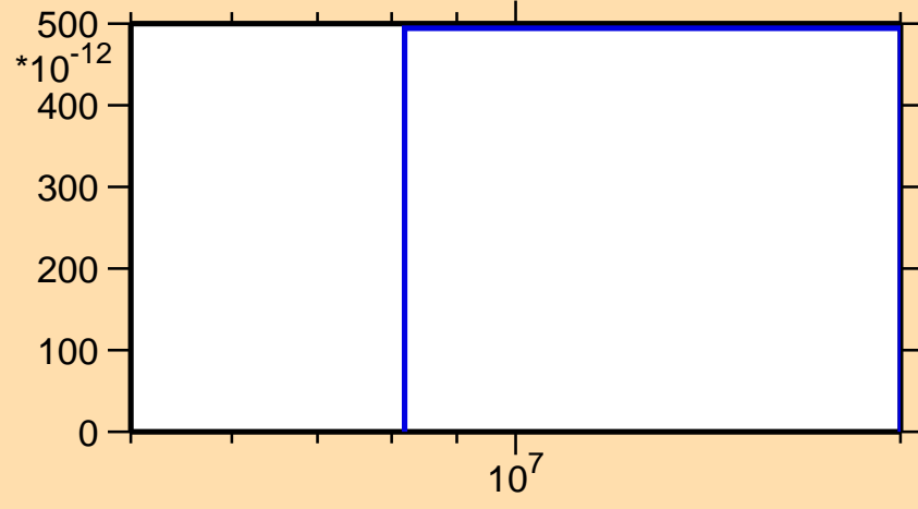
\sigma vs. E for ^{114}\text{Sb}(\text{mt } 45)
