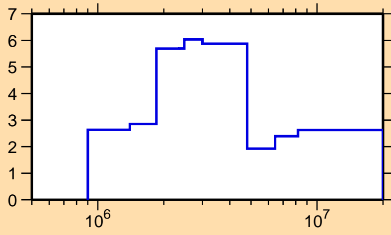
\Delta\sigma/\sigma vs. E for ^{114}\text{Sb}(n, \text{tot.})
