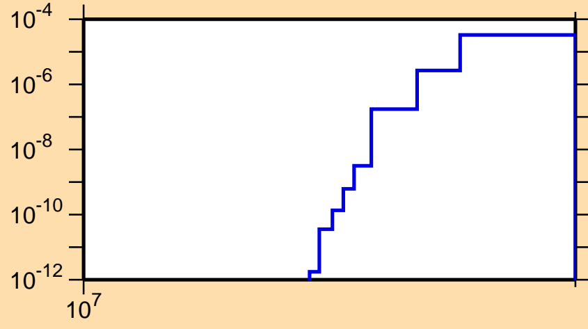
\sigma vs. E for ^{115}\text{Sb}(n,\text{nd})
