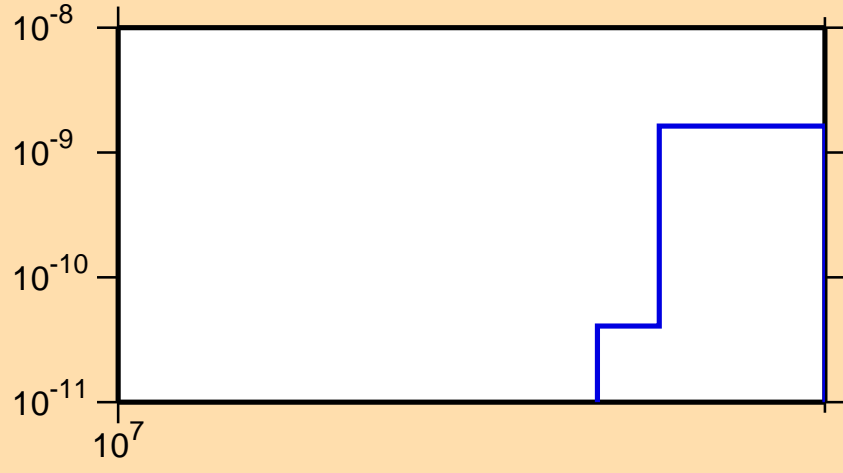
\sigma vs. E for ^{115}\text{Sb}(n,\text{pd})
