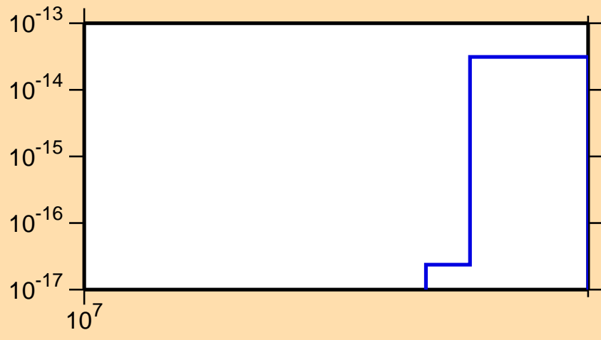
\sigma vs. E for ^{115}\text{Sb}(n,\text{pt})
