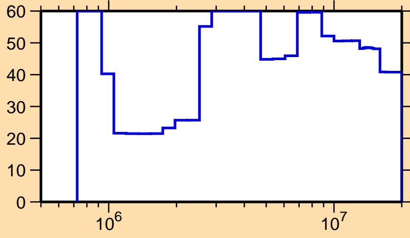
\Delta\sigma/\sigma vs. E for ^{115}\text{Sb}(n,n_1)
