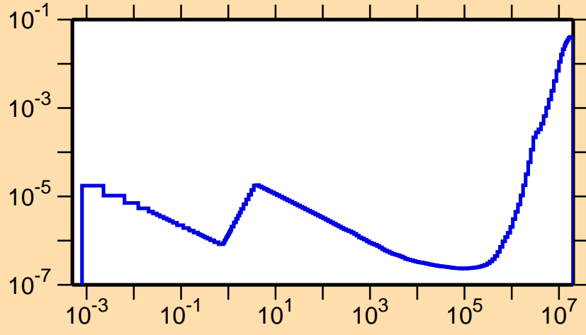
\sigma vs. E for ^{115}\text{Sb}(n,\alpha)
