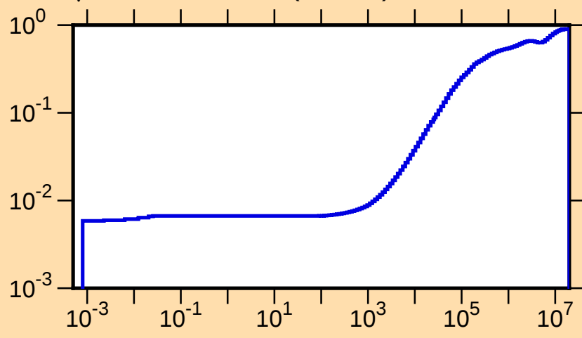
\mu vs. E for ^{116}\text{Sb}(\text{mt251})
