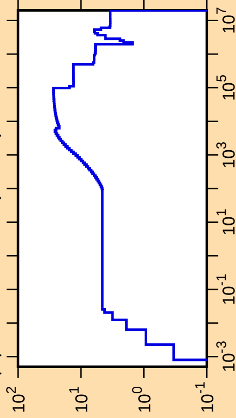
\Delta\mu/\mu vs. E for ^{116}\text{Sb}(\text{mt251})
