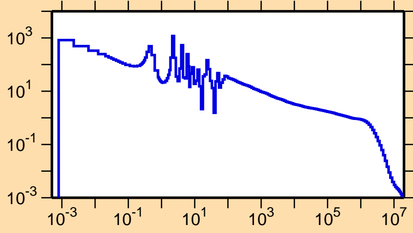
\sigma vs. E for ^{116}\text{Sb}(n,\gamma)
