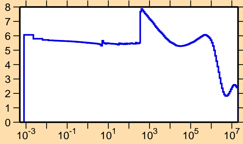
\sigma vs. E for ^{117}\text{Sb}(n,\text{el.})
