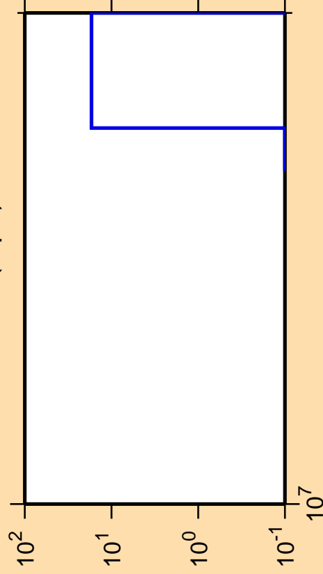
\Delta\sigma/\sigma vs. E for ^{117}\text{Sb}(n,pd)
