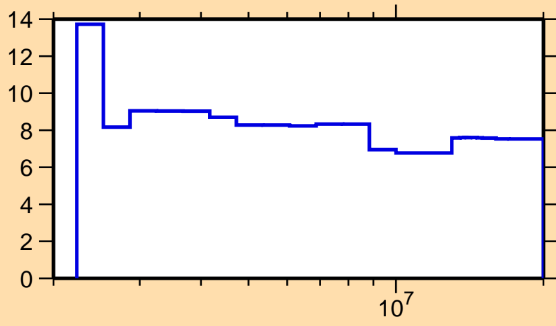
\Delta\sigma/\sigma vs. E for ^{117}\text{Sb}(n,n\text{onel.})
