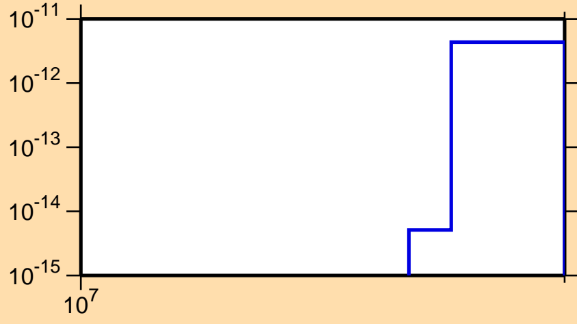
\sigma vs. E for ^{117}\text{Sb}(n,pd)
