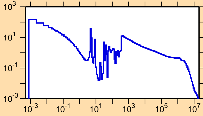
\sigma vs. E for ^{117}\text{Sb}(n,\gamma)
