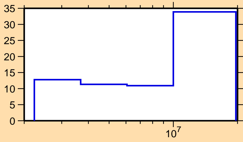
\Delta\sigma/\sigma vs. E for ^{117}\text{Sb}(n,n\text{cont.})
