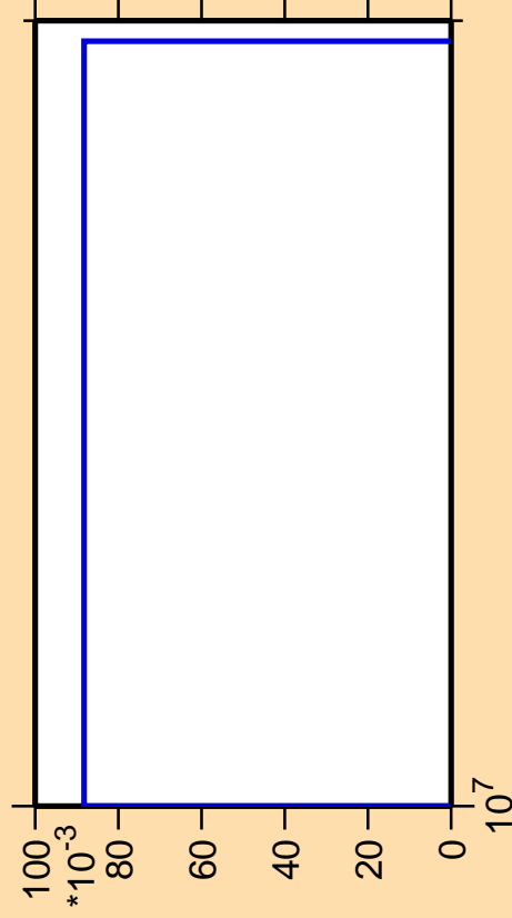
\Delta\sigma/\sigma vs. E for ^{117}\text{Sb}(\text{mt } 45)
