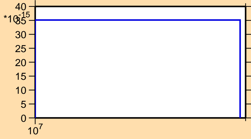
\sigma vs. E for ^{117}\text{Sb}(\text{mt } 45)
