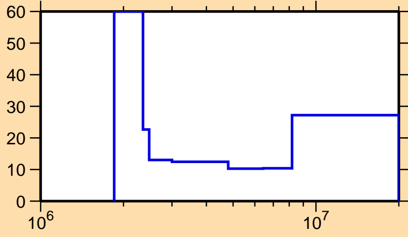
\Delta\sigma/\sigma vs. E for ^{117}\text{Sb}(n,n\text{cont.})
