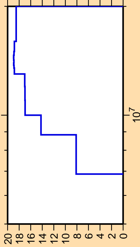
\Delta\sigma/\sigma vs. E for ^{118}\text{Sb}(n, n_{\text{cont}})
