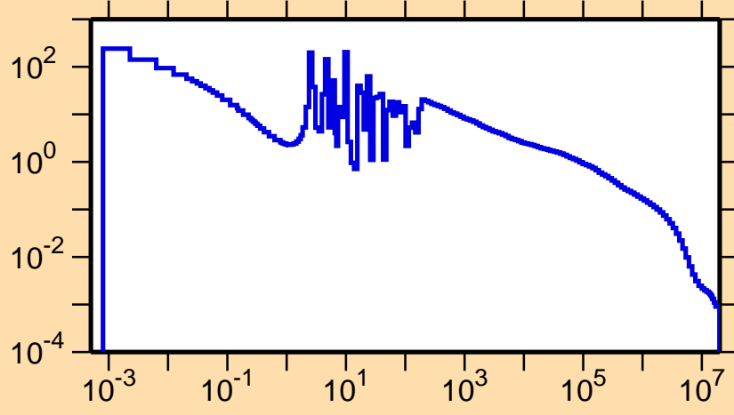
\sigma vs. E for ^{118}\text{Sb}(n,\gamma)
