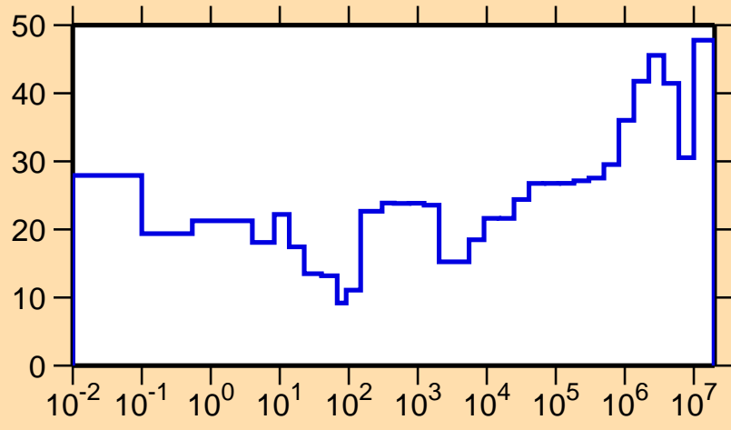
\Delta\sigma/\sigma vs. E for ^{118}\text{Sb}(n,\gamma)
