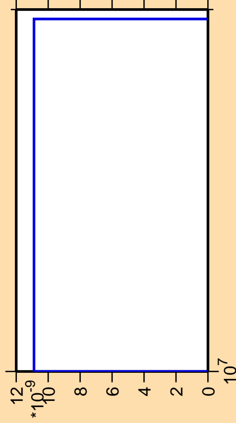
\Delta\sigma/\sigma vs. E for ^{118}\text{Sb} (mt 11)
