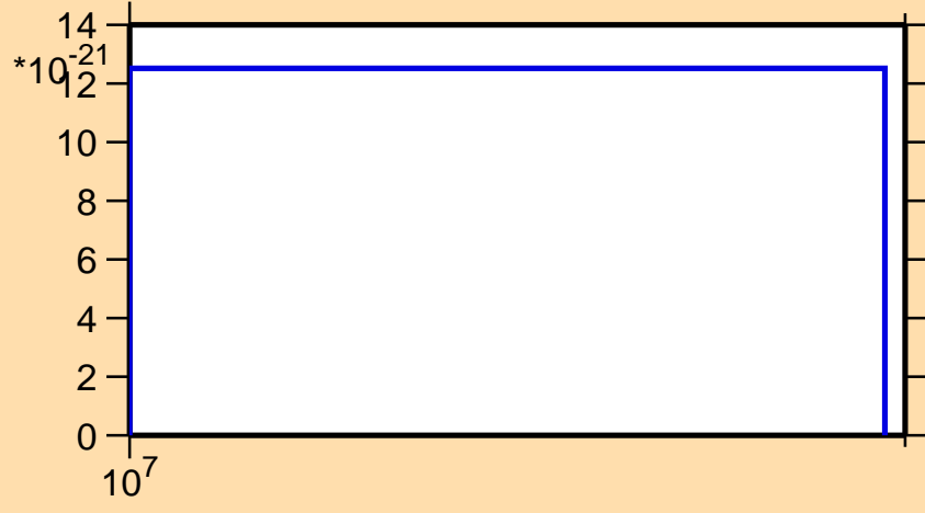
\sigma vs. E for ^{118}\text{Sb} (mt 11)
