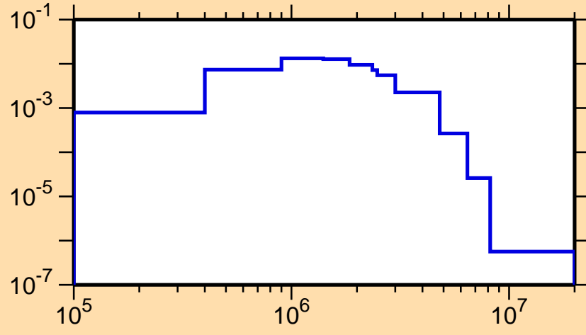
\sigma vs. E for ^{118}\text{Sb}(n,n_4)
