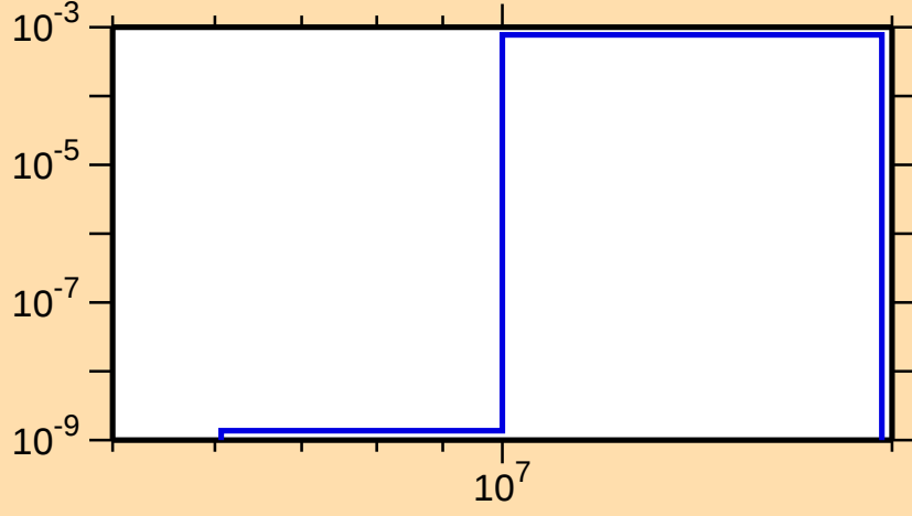
\sigma vs. E for ^{118}\text{Sb}(n,t)
