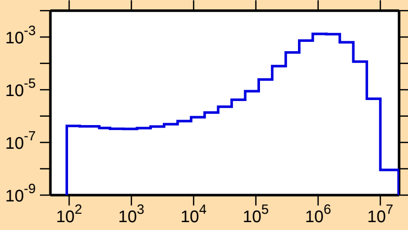
\sigma vs. E for ^{118}\text{Sb}(n,n_3)
