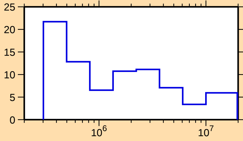
\Delta\sigma/\sigma vs. E for ^{118}\text{Sb}(n,\text{tot.})
