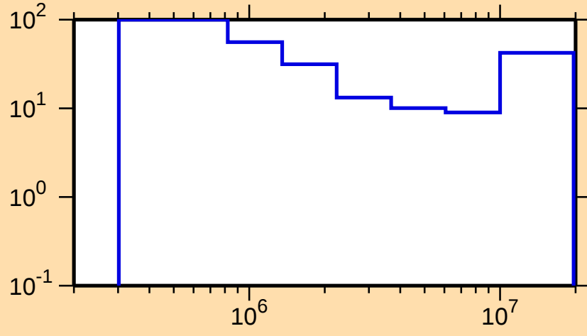
\Delta\sigma/\sigma vs. E for ^{118}\text{Sb}(n,n\text{cont.})
