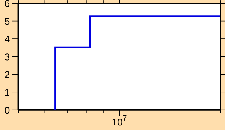
\Delta\sigma/\sigma vs. E for ^{118}\text{Sb}(n,\text{tot.})
