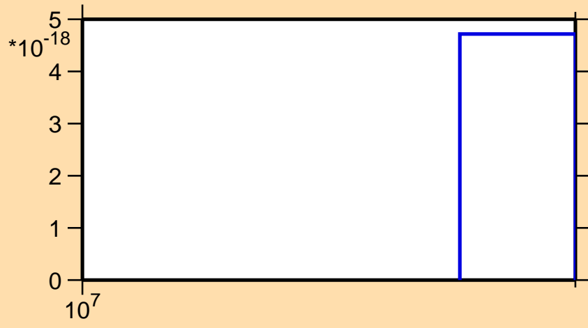
\sigma vs. E for ^{119}\text{Sb} (mt 11)
