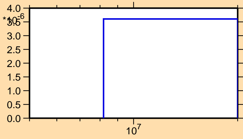
\sigma vs. E for ^{120}\text{Sb}(n,nd)
