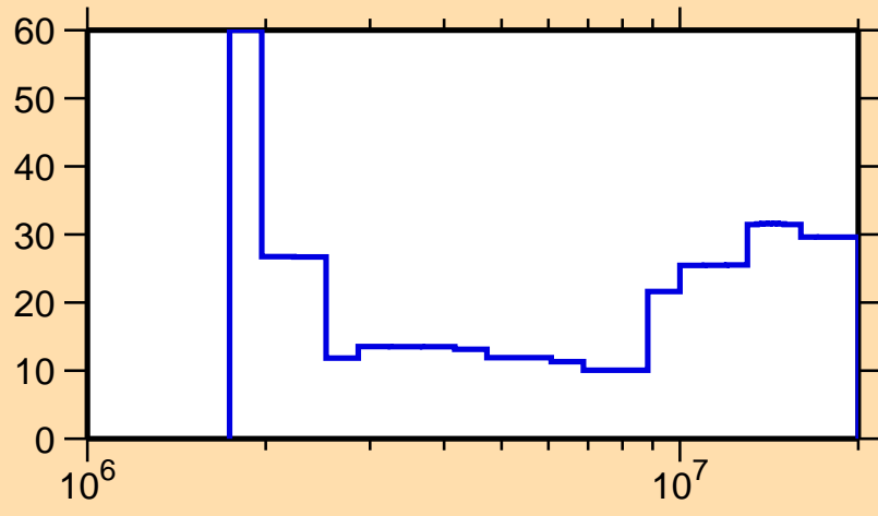
\Delta\sigma/\sigma vs. E for ^{121}\text{Sb}(n,n\text{cont.})
