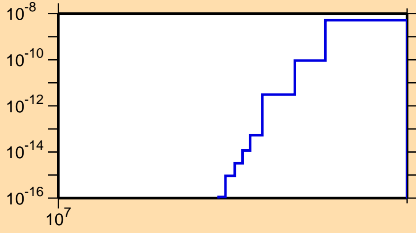
\sigma vs. E for ^{121}\text{Sb}(n,\text{He3})
