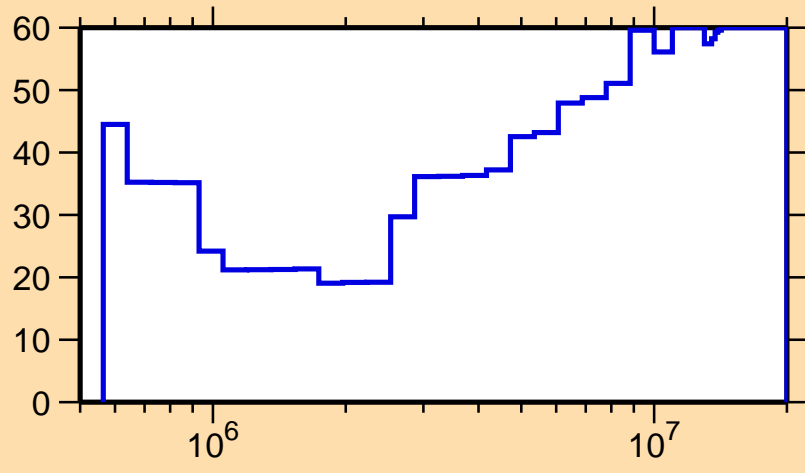
\Delta\sigma/\sigma vs. E for ^{121}\text{Sb}(n,n_1)
