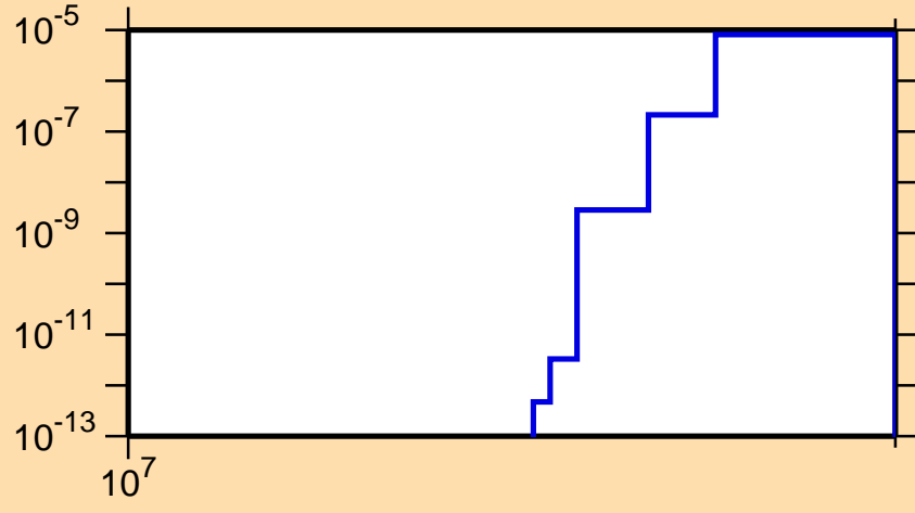
\sigma vs. E for ^{121}\text{Sb}(n,\text{nd})
