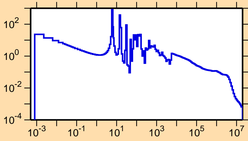
\sigma vs. E for ^{121}\text{Sb}(n,\gamma)
