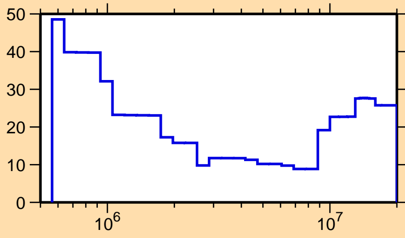
\Delta\sigma/\sigma vs. E for ^{121}\text{Sb}(n,\text{inel.})
