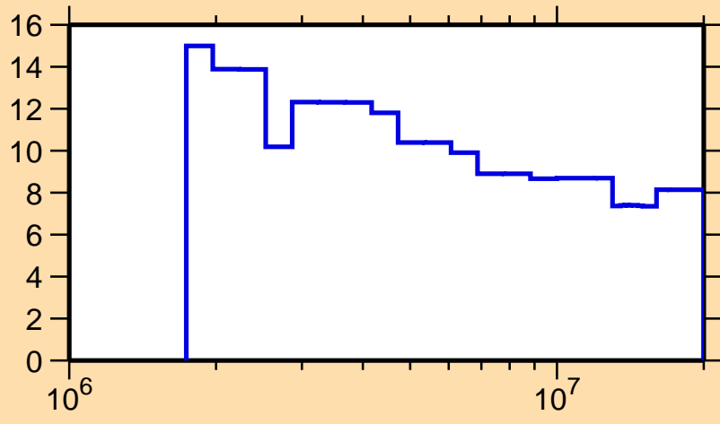
\Delta\sigma/\sigma vs. E for ^{121}\text{Sb}(n,\text{nonel.})
