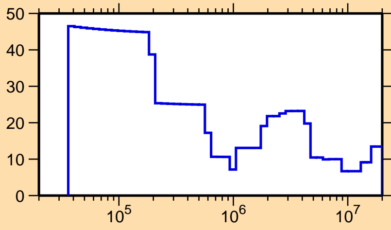
\Delta\sigma/\sigma vs. E for ^{121}\text{Sb}(n,\text{el.})
