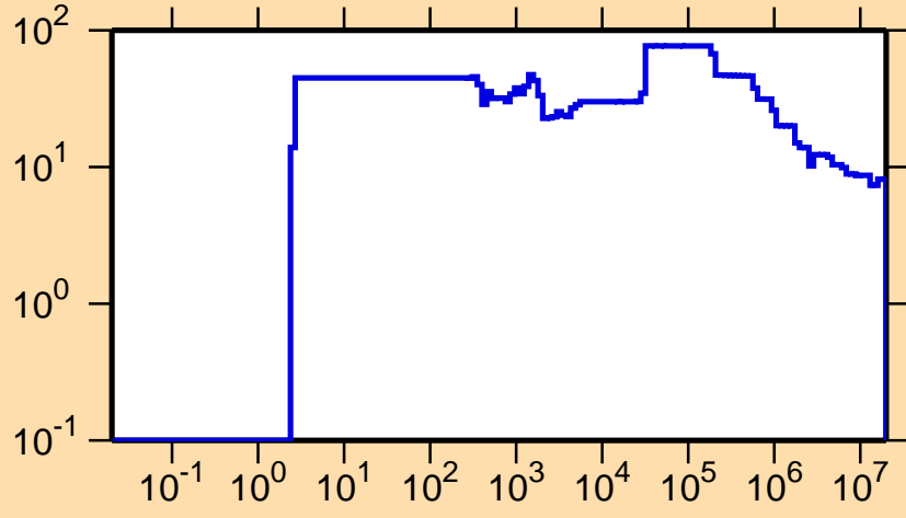
\Delta\sigma/\sigma vs. E for ^{121}\text{Sb}(n,\text{nonel.})
