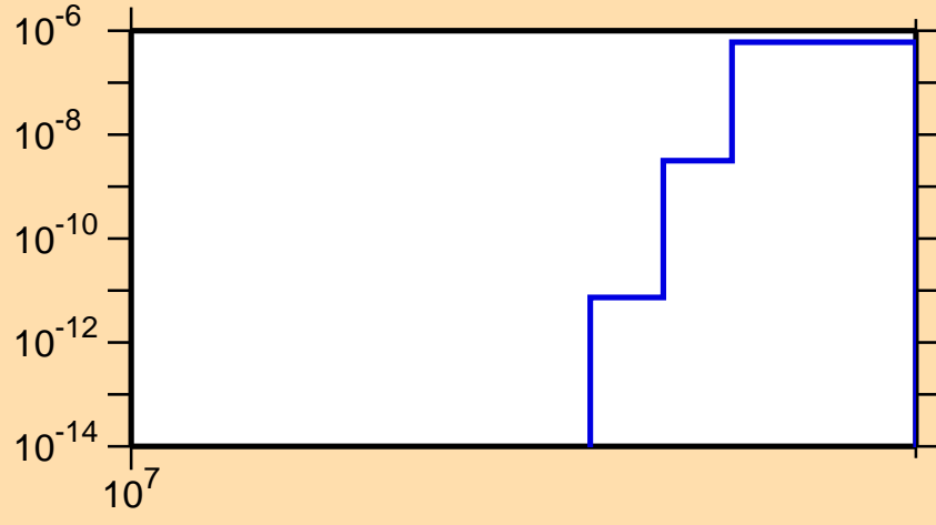
\sigma vs. E for ^{121}\text{Sb}(n,nt)
