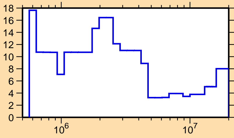
\Delta\sigma/\sigma vs. E for ^{121}\text{Sb}(n,\text{tot.})
