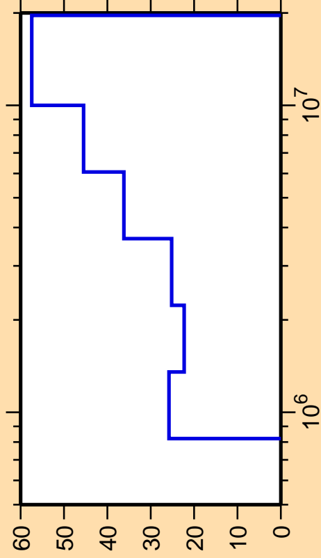
\Delta\sigma/\sigma vs. E for ^{121}\text{Sb}(n,n_4)
