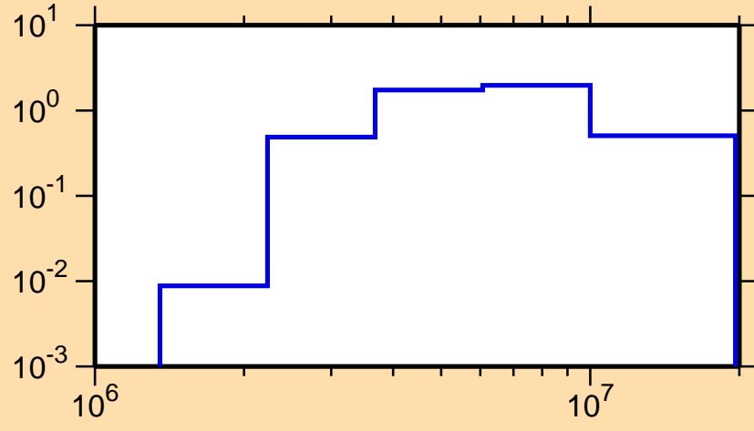
\sigma vs. E for ^{121}\text{Sb}(n,n\text{cont.})
