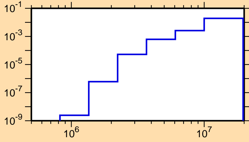
\sigma vs. E for ^{121}\text{Sb}(n,p)
