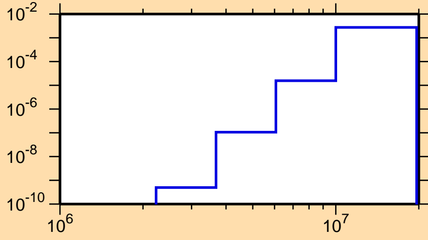
\sigma vs. E for ^{121}\text{Sb}(n,\alpha)
