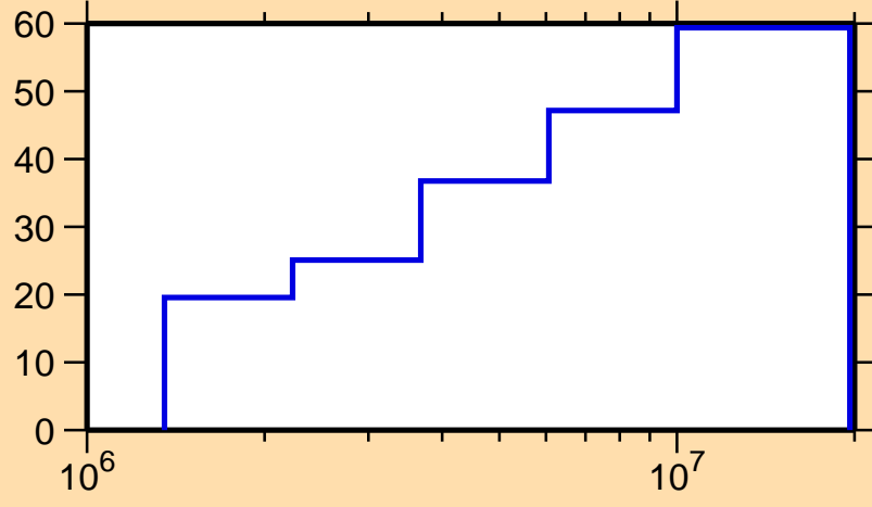
\Delta\sigma/\sigma vs. E for ^{121}\text{Sb}(n, n_1)
