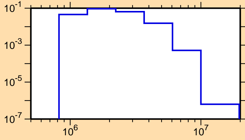
\sigma vs. E for ^{121}\text{Sb}(n,n_4)
