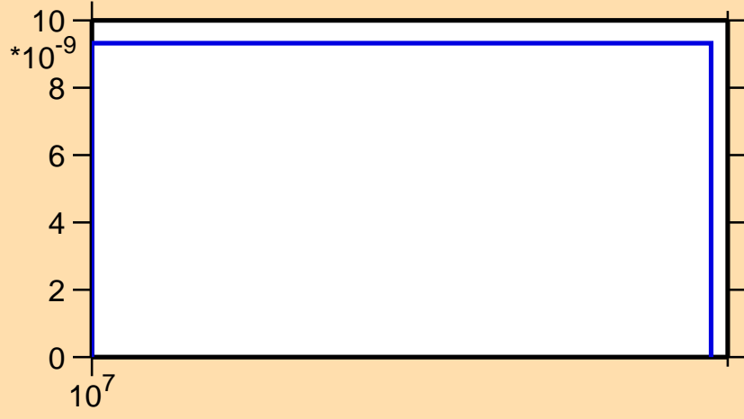
\sigma vs. E for ^{121}\text{Sb}(n,2np)
