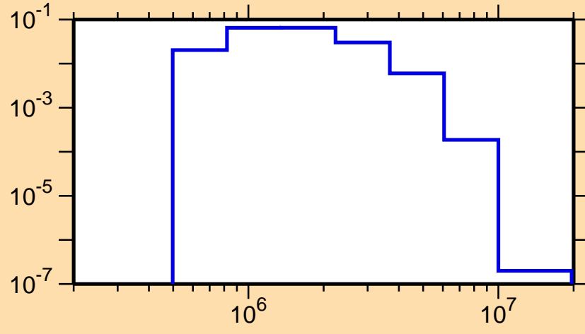
\sigma vs. E for ^{121}\text{Sb}(n,n_3)
