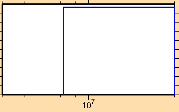
\sigma vs. E for ^{121}\text{Sb}(n,t)
