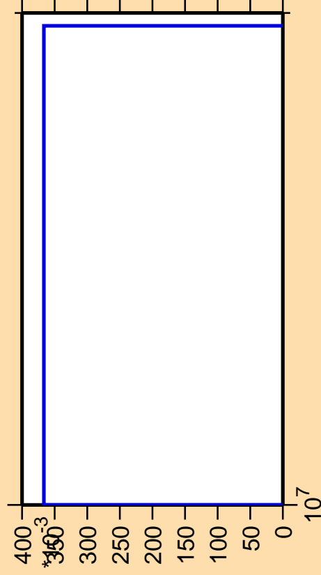
\Delta\sigma/\sigma vs. E for ^{124}\text{Sb}(n,\text{He3})
