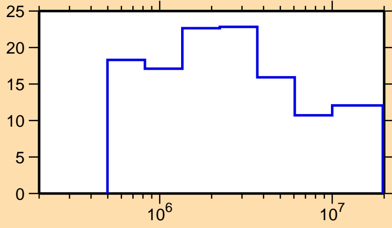
\Delta\sigma/\sigma vs. E for ^{124}\text{Sb}(n,el.)
