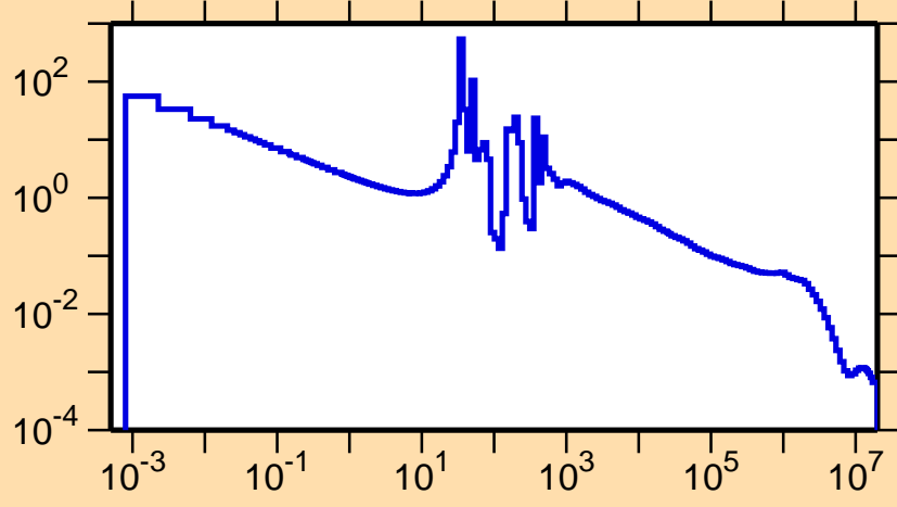
\sigma vs. E for ^{125}\text{Sb}(n,\gamma)
