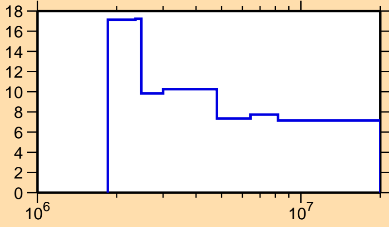
\Delta\sigma/\sigma vs. E for ^{125}\text{Sb}(n,\text{nonel.})
