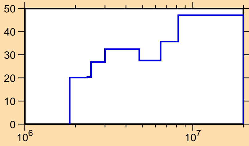
\Delta\sigma/\sigma vs. E for ^{125}\text{Sb}(n, n_1)
