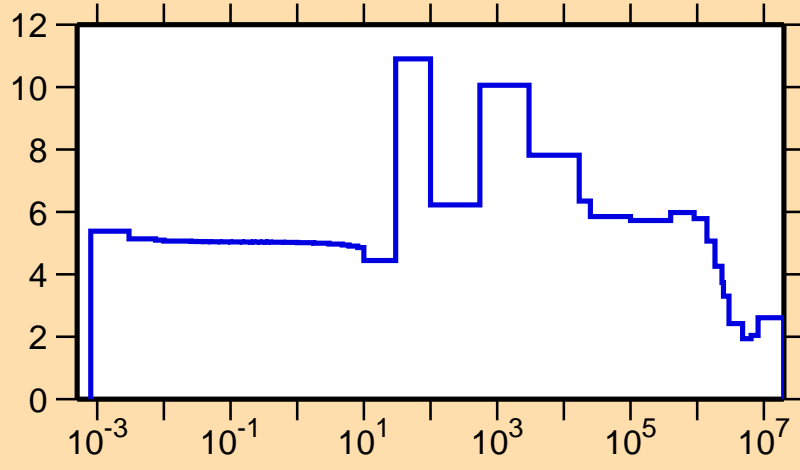
\sigma vs. E for ^{125}\text{Sb}(n,\text{el.})
