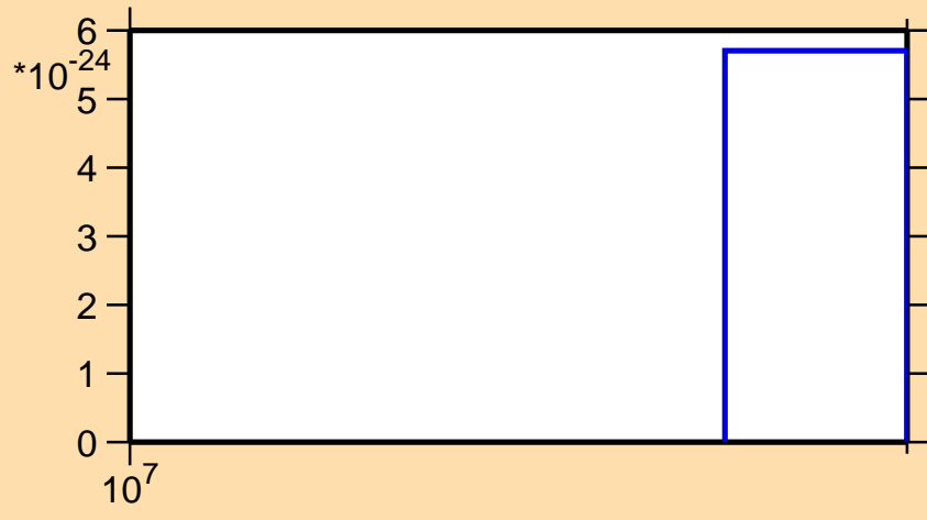
\sigma vs. E for ^{126}\text{Sb} (mt 11)
