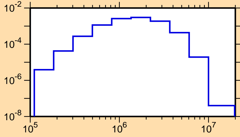
\sigma vs. E for ^{126}\text{Sb}(n,n_4)
