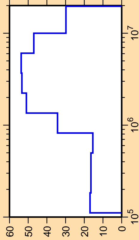
\Delta\sigma/\sigma vs. E for ^{126}\text{Sb}(n,n_4)
