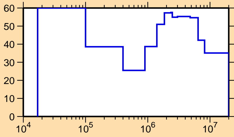
\Delta\sigma/\sigma vs. E for ^{126}\text{Sb}(n,n_1)
