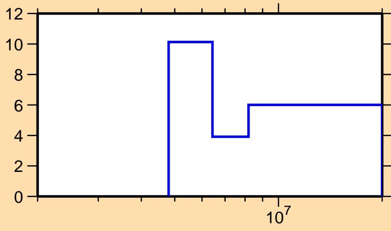
\Delta\sigma/\sigma vs. E for ^{126}\text{Sb}(n,\text{tot.})
