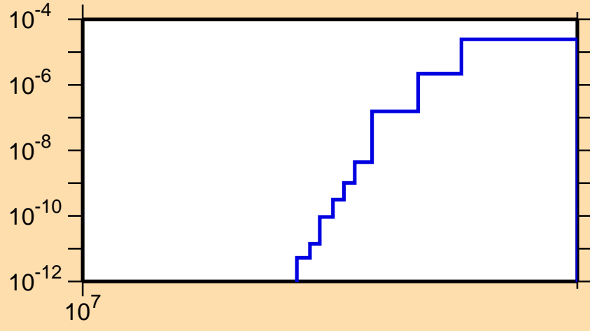
\sigma vs. E for ^{126}\text{Sb}(n,nd)
