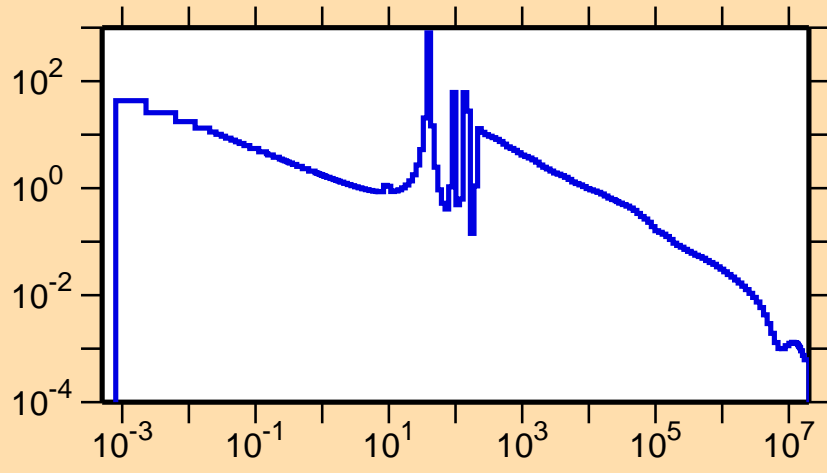
\sigma vs. E for ^{126}\text{Sb}(n,\gamma)
