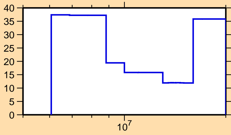
\Delta\sigma/\sigma vs. E for ^{126}\text{Sb}(n,2n)
