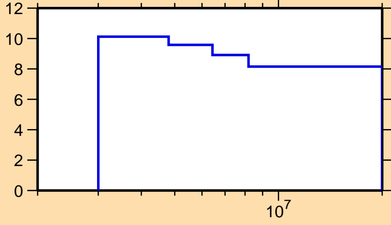
\Delta\sigma/\sigma vs. E for ^{128}\text{Sb}(n,\text{nonel.})
