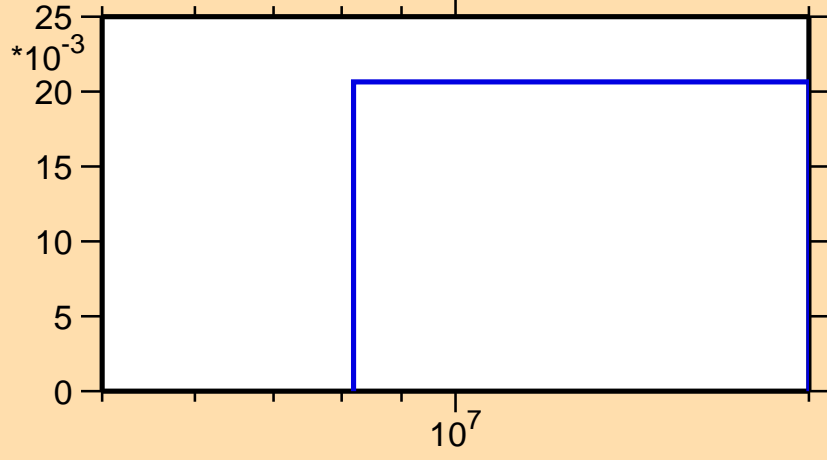
\sigma vs. E for ^{128}\text{Sb}(n,3n)
