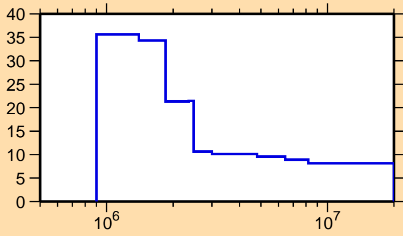
\Delta\sigma/\sigma vs. E for ^{128}\text{Sb}(n,\text{nonel.})
