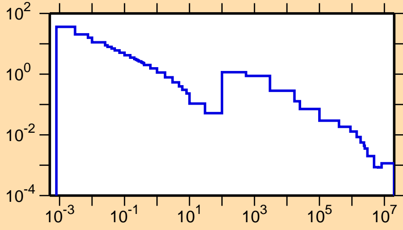
\sigma vs. E for ^{128}\text{Sb}(n,\gamma)
