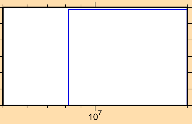
\sigma vs. E for ^{128}\text{Sb}(n,nd)
