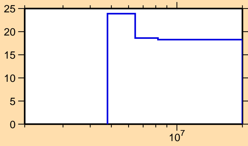
\Delta\sigma/\sigma vs. E for ^{128}\text{Sb}(n,\text{el.})
