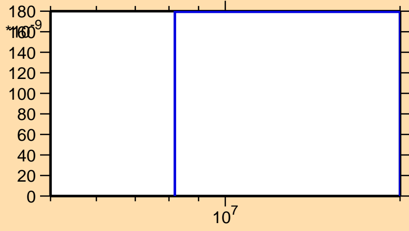
\sigma vs. E for ^{128}\text{Sb}(n,n\alpha)
