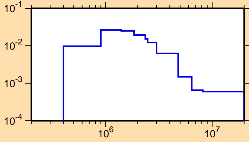
\sigma vs. E for ^{128}\text{Sb}(n,n_3)
