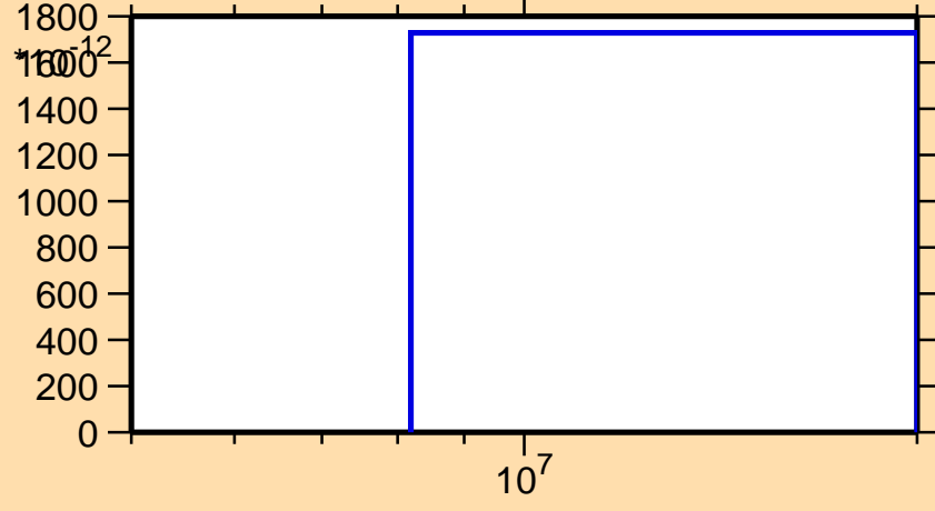
\sigma vs. E for ^{128}\text{Sb}(n,2np)
