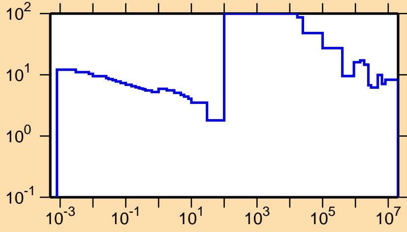
\Delta\sigma/\sigma vs. E for ^{128}\text{Sb}(n,\text{tot.})
