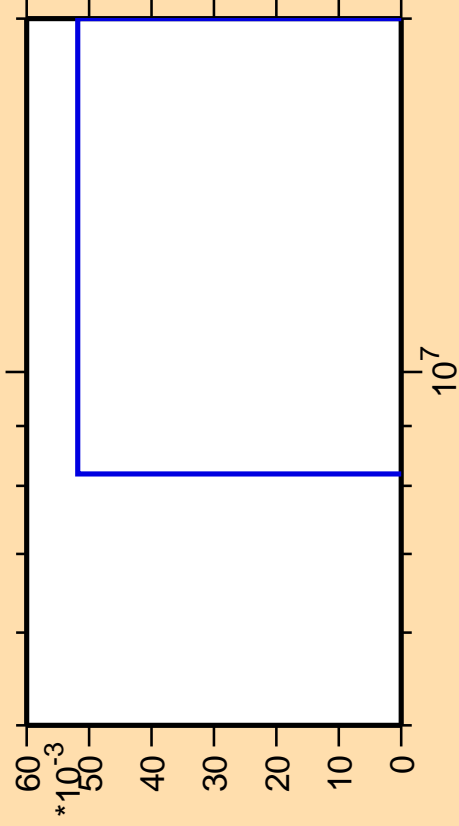
\Delta\sigma/\sigma vs. E for ^{128}\text{Sb}(n,2n\alpha)
