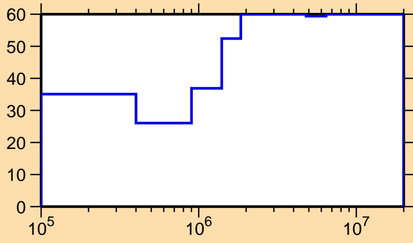
\Delta\sigma/\sigma vs. E for ^{128}\text{Sb}(n,n_1)
