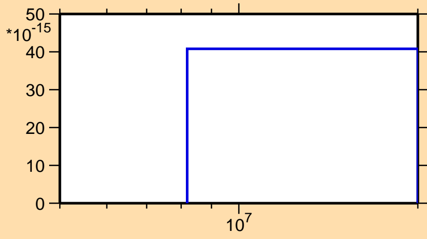
\sigma vs. E for ^{128}\text{Sb}(n,2n\alpha)
