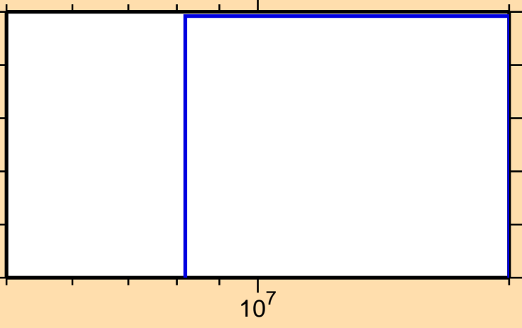
\sigma vs. E for ^{128}\text{Sb}(n,np)
