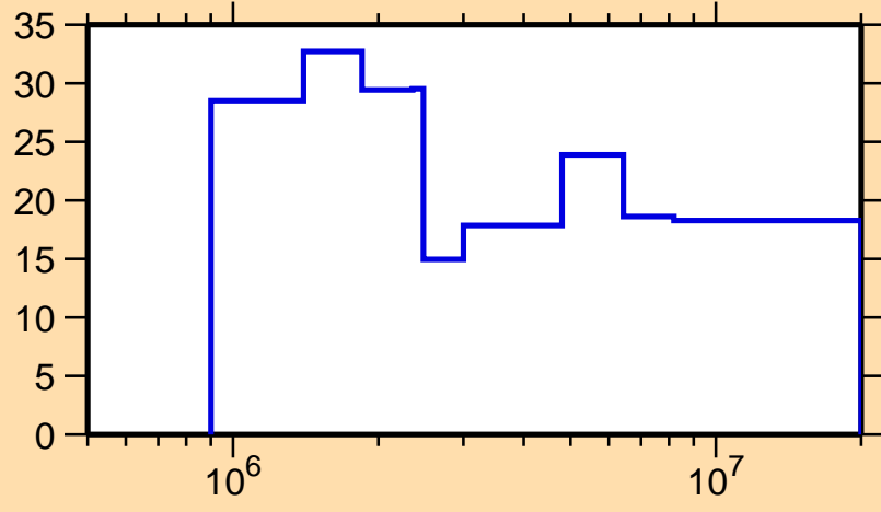
\Delta\sigma/\sigma vs. E for ^{128}\text{Sb}(n,\text{el.})
