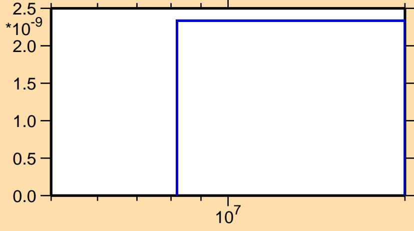
\sigma vs. E for ^{128}\text{Sb}(n,nt)
