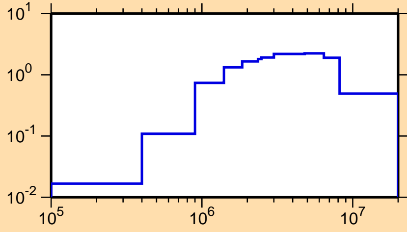
\sigma vs. E for ^{128}\text{Sb}(n,\text{inel.})
