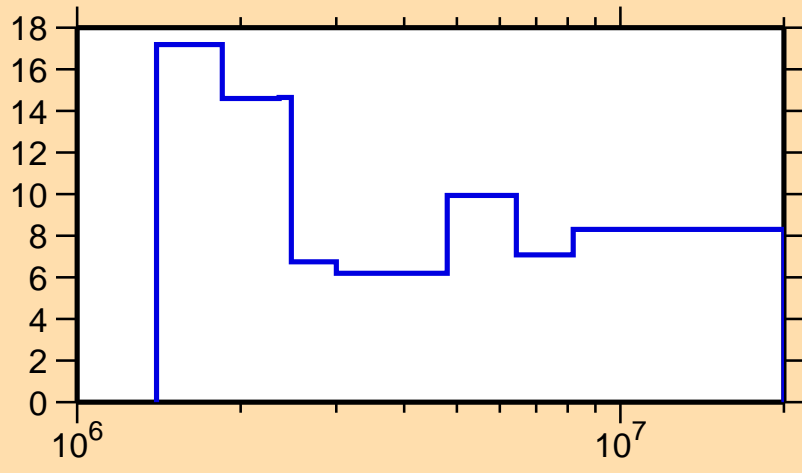
\Delta\sigma/\sigma vs. E for ^{128}\text{Sb}(n,\text{tot.})
