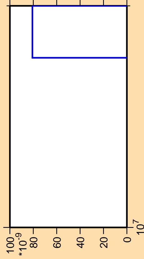
\Delta\sigma/\sigma vs. E for ^{128}\text{Sb} (mt 11)
