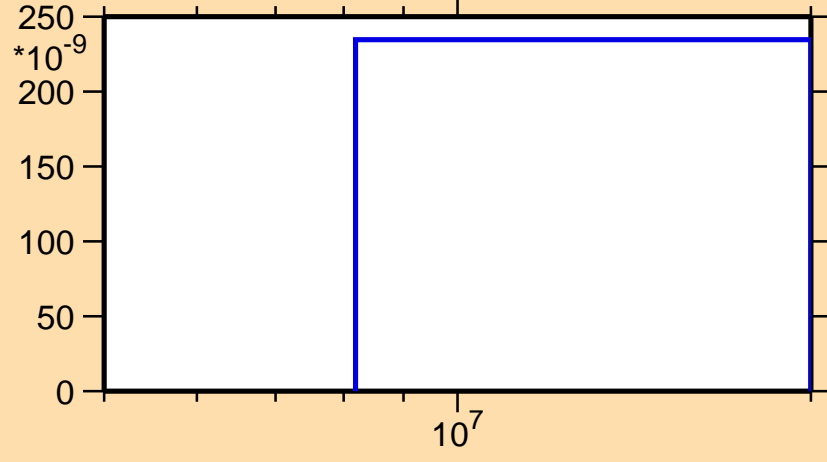
\sigma vs. E for ^{128}\text{Sb}(n,n\alpha)
