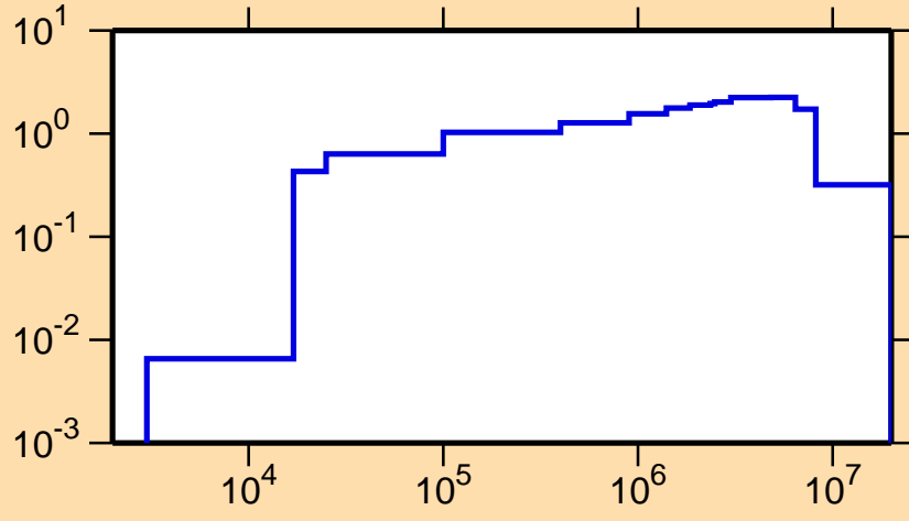
\sigma vs. E for ^{129}\text{Sb}(n,\text{inel.})
