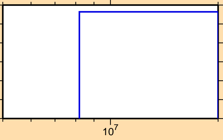
\sigma vs. E for ^{129}\text{Sb}(n,nt)
