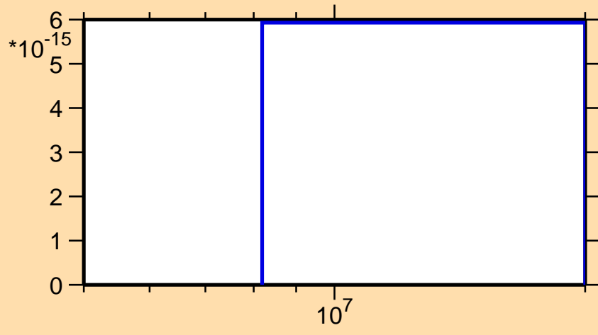
\sigma vs. E for ^{129}\text{Sb}(n,2n\alpha)
