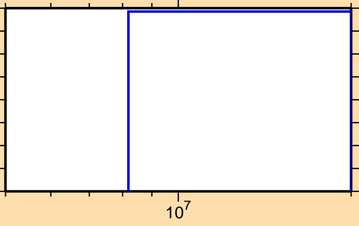
\sigma vs. E for ^{129}\text{Sb}(n,3n)
