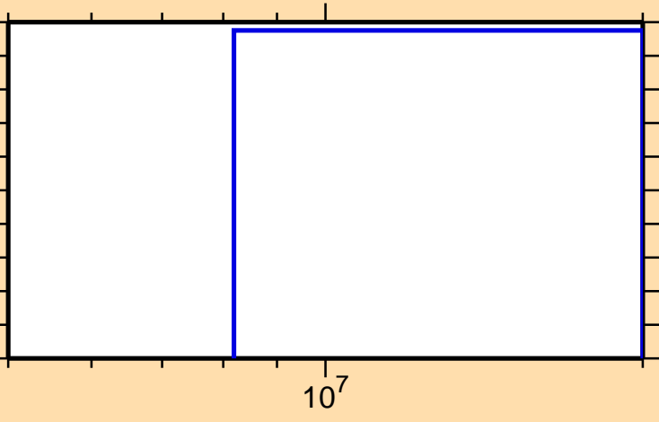
\sigma vs. E for ^{130}\text{Sb}(n,d)
