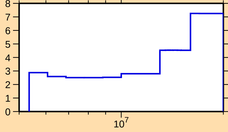
\Delta\sigma/\sigma vs. E for ^{130}\text{Sb}(n,\text{tot.})
