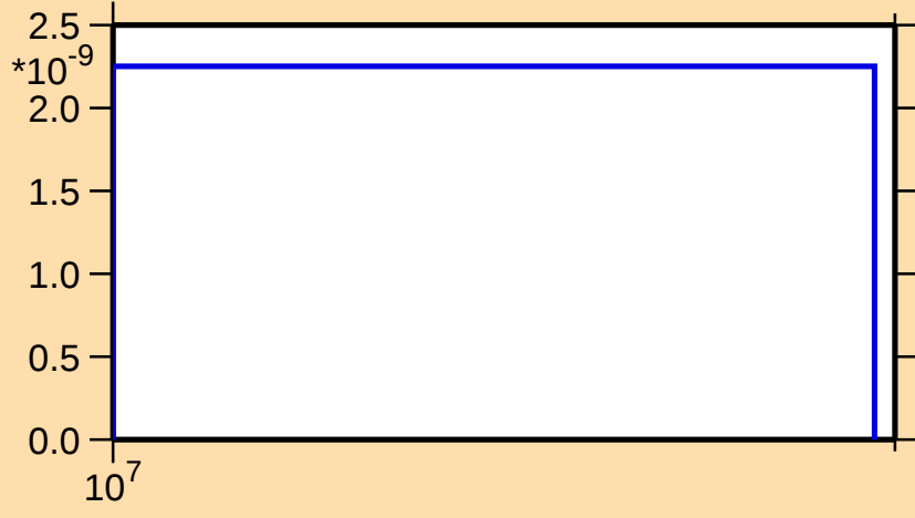
\sigma vs. E for ^{130}\text{Sb}(n,nt)
