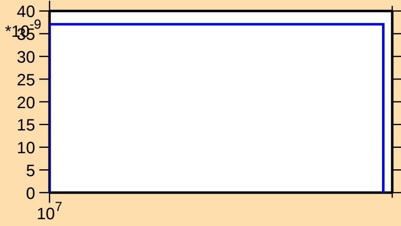
\sigma vs. E for ^{130}\text{Sb}(n,n\alpha)
