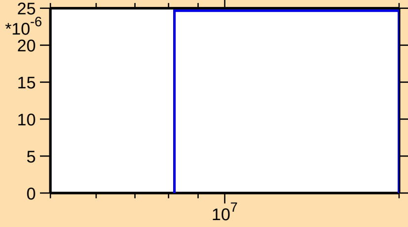
\sigma vs. E for ^{130}\text{Sb}(n,t)
