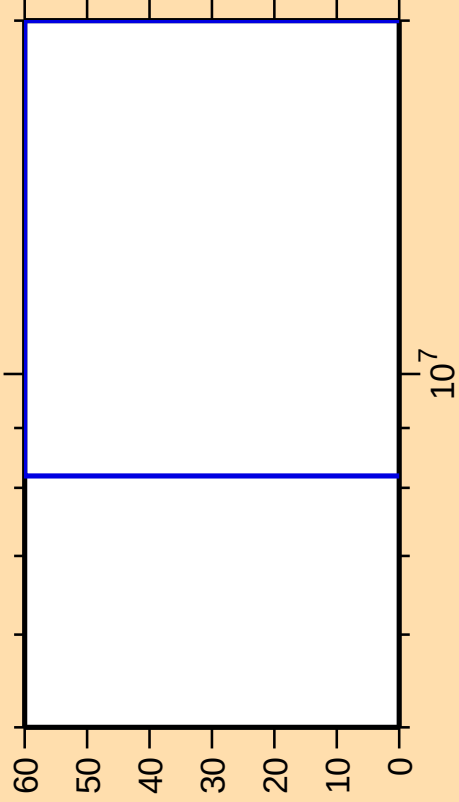
\Delta\sigma/\sigma vs. E for ^{130}\text{Sb}(n,t)
