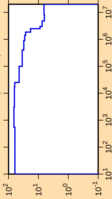
\Delta\sigma/\sigma vs. E for ^{130}\text{Sb}(n,\text{nonel.})
