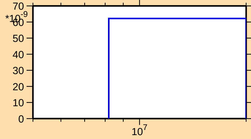
\sigma vs. E for ^{130}\text{Sb}(n,\text{nd})
