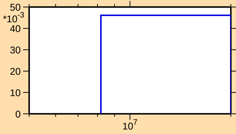
\sigma vs. E for ^{130}\text{Sb}(n,3n)
