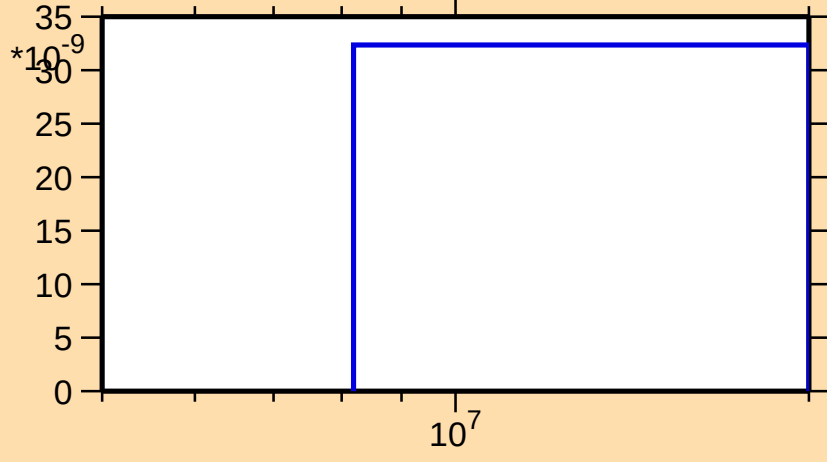
\sigma vs. E for ^{130}\text{Sb}(n,n\alpha)
