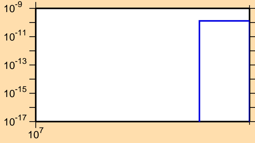
\sigma vs. E for ^{131}\text{Sb}(n,2np)
