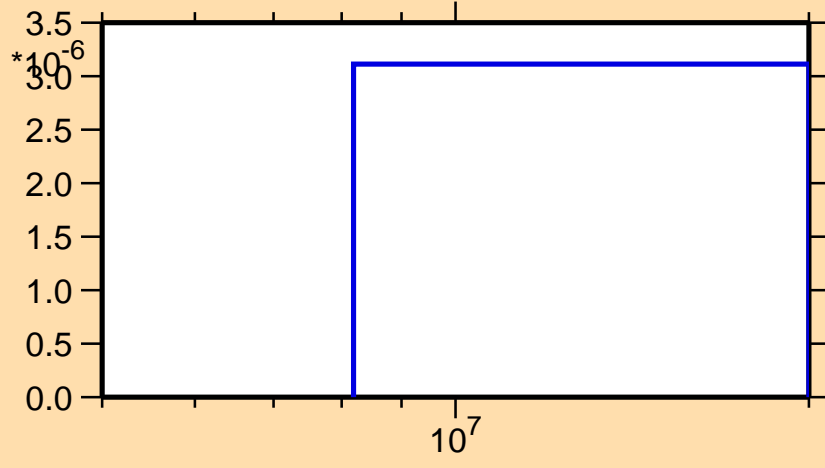
\sigma vs. E for ^{131}\text{Sb}(n,t)
