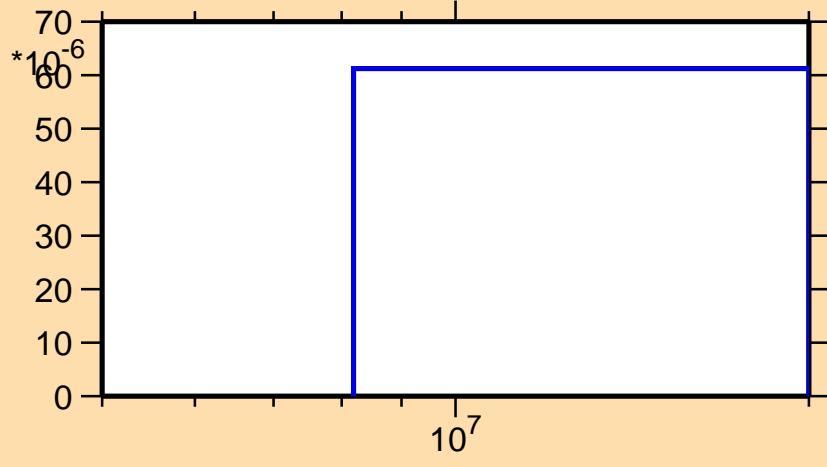
\sigma vs. E for ^{131}\text{Sb}(n,np)
