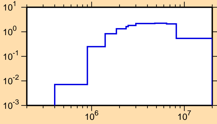
\sigma vs. E for ^{131}\text{Sb}(n,\text{inel.})
