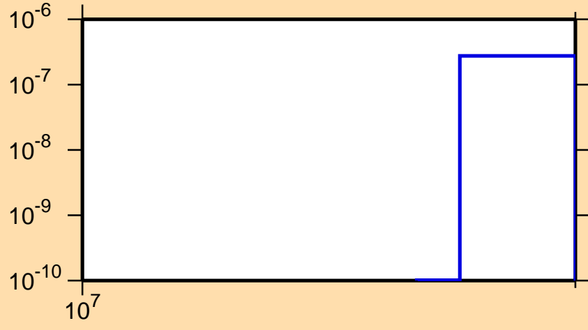
\sigma vs. E for ^{132}\text{Sb}(n,nt)
