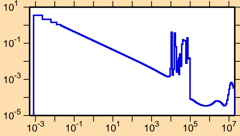
\sigma vs. E for ^{132}\text{Sb}(n,\gamma)
