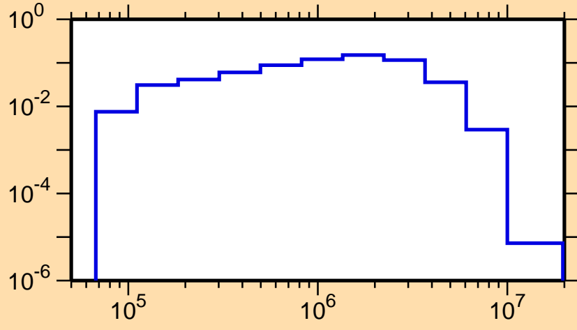
\sigma vs. E for ^{132}\text{Sb}(n,n_3)
