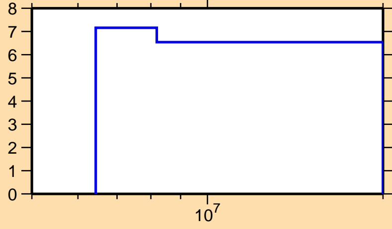
\Delta\sigma/\sigma vs. E for ^{132}\text{Sb}(n,\text{el.})
