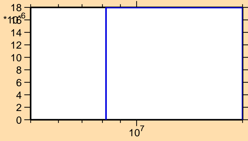
\sigma vs. E for ^{132}\text{Sb}(n,t)
