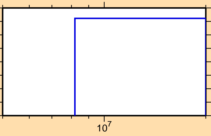
\sigma vs. E for ^{132}\text{Sb}(n,3n)
