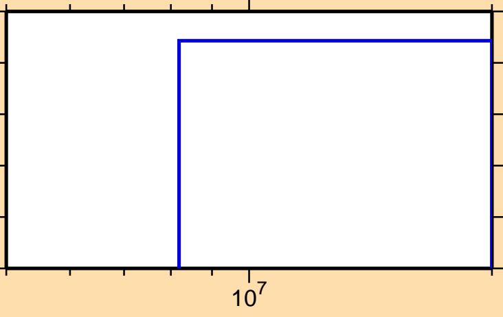
\sigma vs. E for ^{132}\text{Sb}(n,n\alpha)
