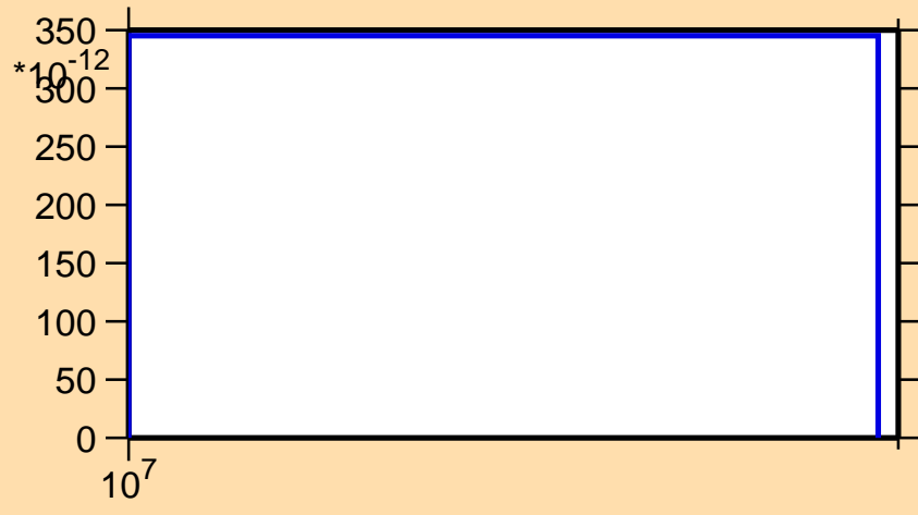
\sigma vs. E for ^{133}\text{Sb}(n,n\alpha)
