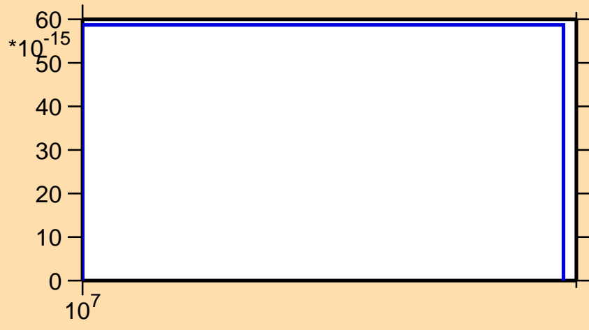
\sigma vs. E for ^{133}\text{Sb}(n,2np)
