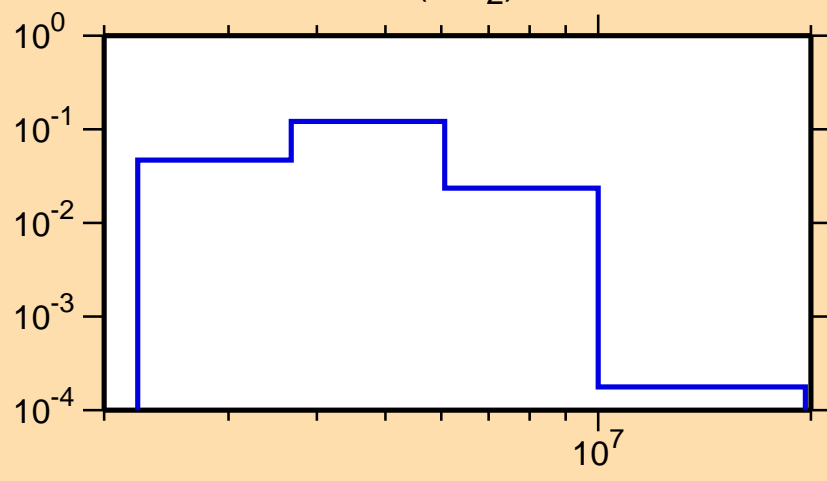
\sigma vs. E for ^{133}\text{Sb}(n,n_2)
