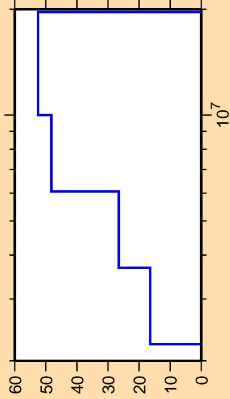
\Delta\sigma/\sigma vs. E for ^{133}\text{Sb}(n,n_2)
